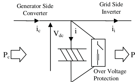
Figure 7. Over voltage protection scheme of DC-link.
