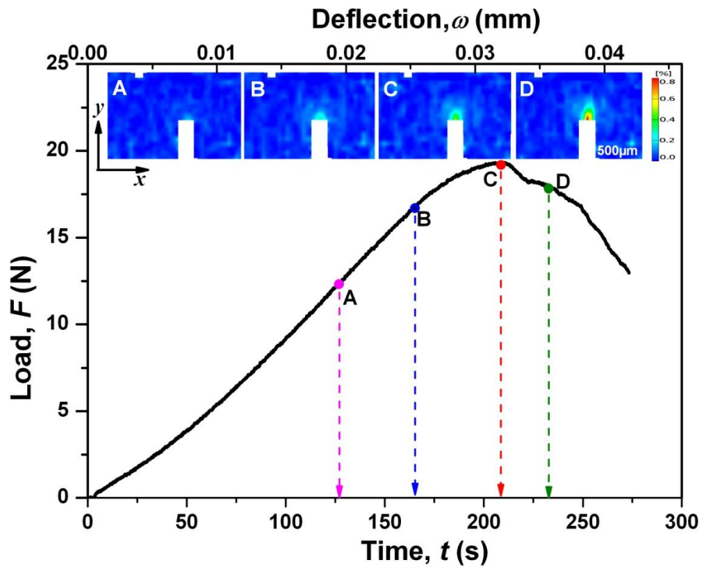
Fig. 3 A typical loading-deflection-time curve of 8YSZ samples during SENB. A series of strain mapping (insets A, B, C and D) show the evolution of strain in the monitored area with the increase of bending loads at N = 200 .
