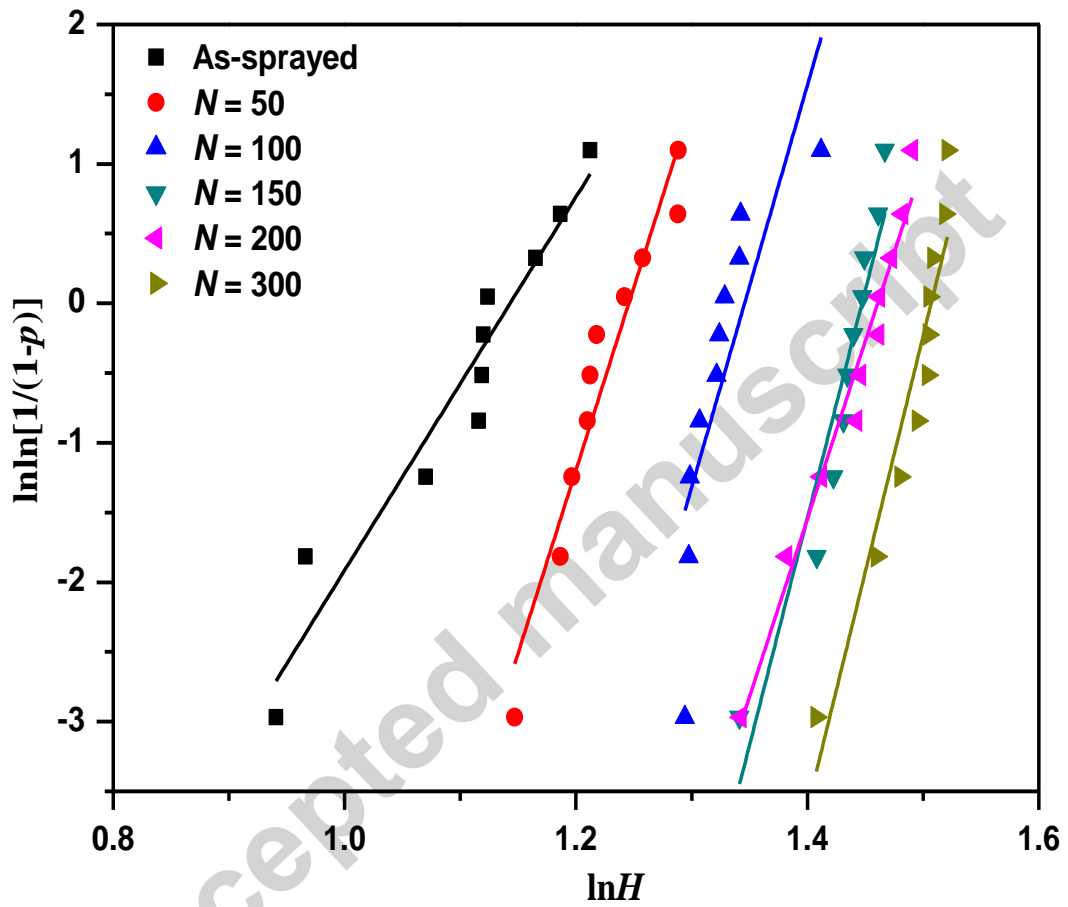
Fig. 7 The Weibull plot of hardness of 8YSZ coatings by Vickers indentations.
