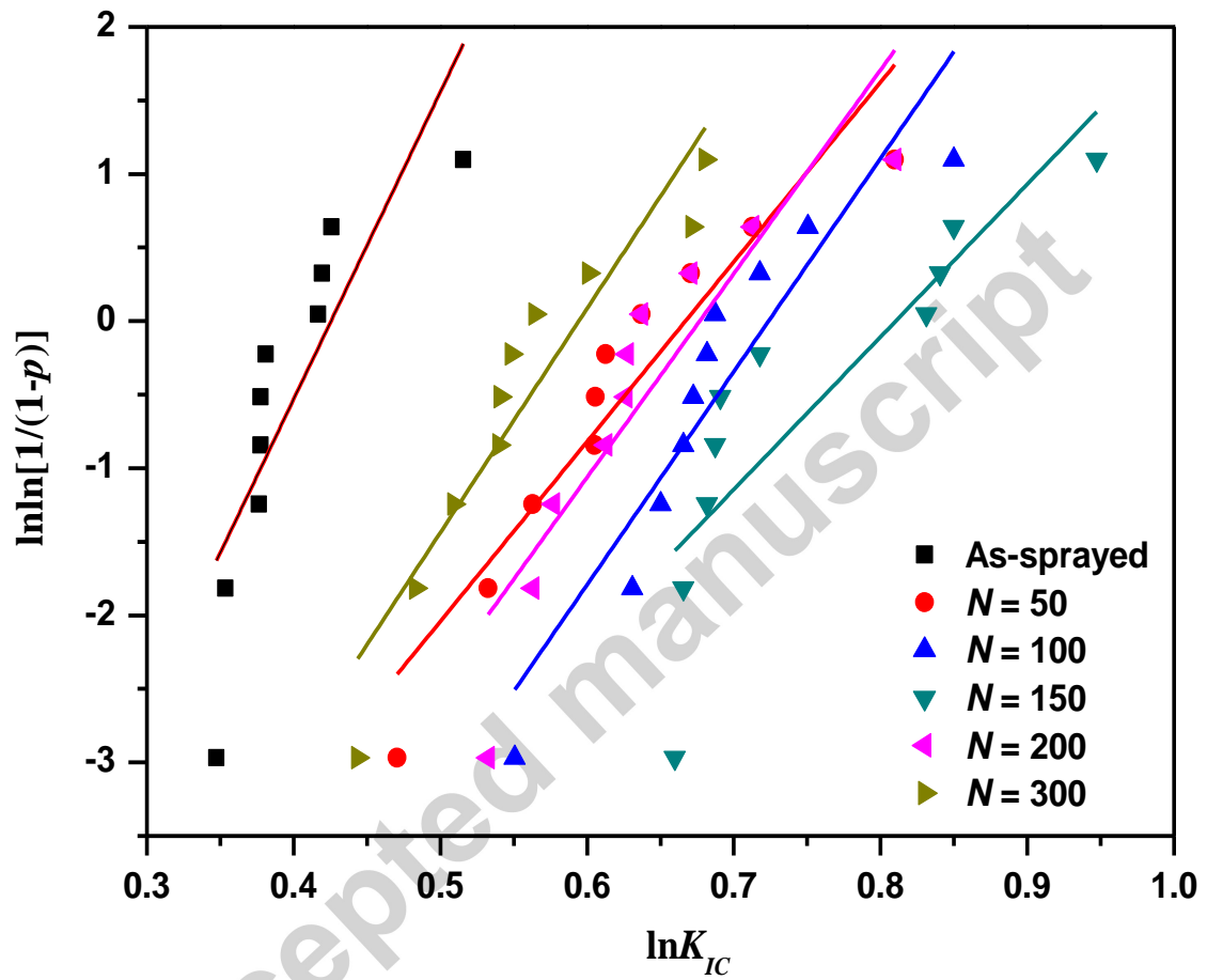
Fig. 8 The Weibull plot of fracture toughness of 8YSZ coatings by Vickers indentations.
