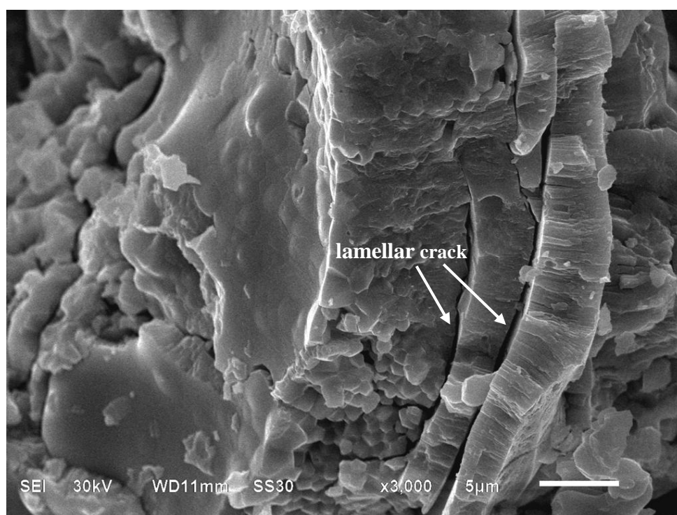
Fig. 5 Typical SEM micrograph of fracture surface of freestanding 8YSZ samples after SENB test, where N = 200 .
