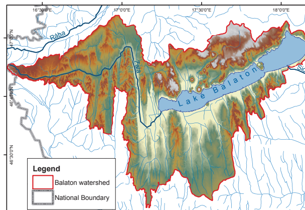
Fig. 1. Lake Balaton and the topography of its watershed. Elevation ranges between 100 and 500 m above sea level.
