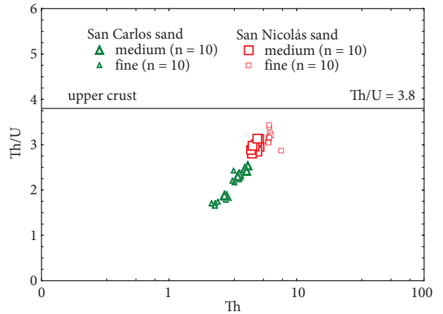
Figure 7. Th/U versus Th bivariate plot for the beach sands.
