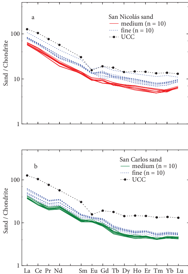
Figure 6. Chondrite-normalized rare earth elements plot. Normalization values are from McDonough and Sun (1995). The average upper continental crust (UCC; Taylor and McLennan, 1985) value is also included for reference. a) San Nicolás; b) San Carlos.
