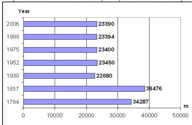
Fig. 5. The length changes of the studied reach of the River Bodrog between 1784 and 2006
