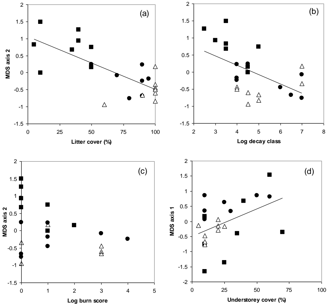
Figure 4. Relationship between MDS ordination scores of community composition and (a) litter cover, (b) log decay class, (c) the proportion of the log's surface area burnt by fire, and (d) cover of understorey plants (■ = 5-year old rehabilitation, ● 15 year old rehabilitation, Δ = unmined forest). Log decay was scored on a 10-point classification from early (1) to advanced (10) stage of decay.
