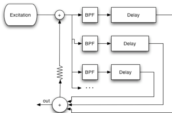
Figure 4. Simple banded waveguide signal flow.
