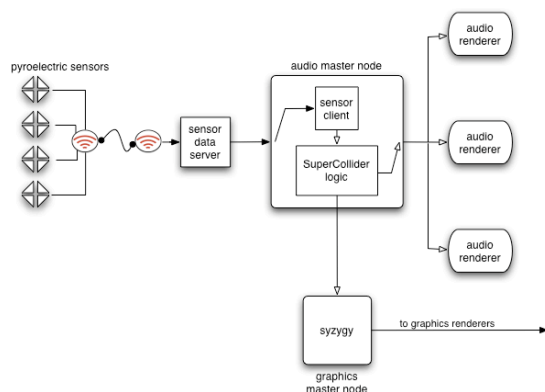
Figure 2. soundSense network topology.
