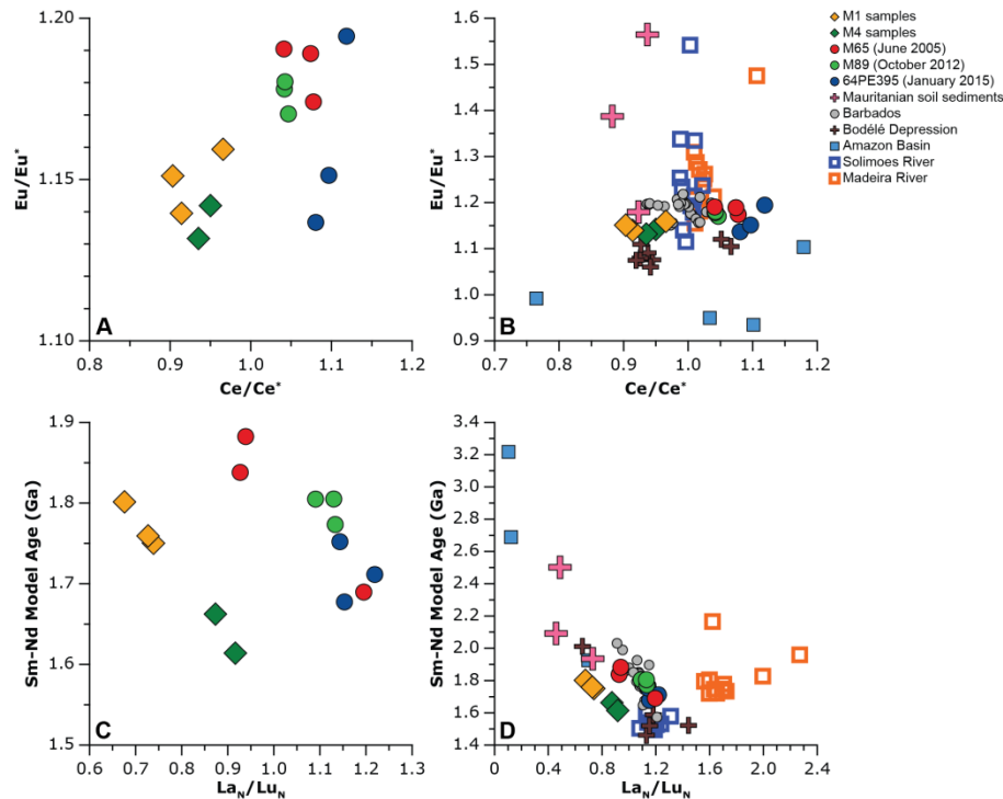
Fig. 6. A: Eu - and Ce -anomalies of samples from sediment traps and shipboard collected aerosols. B: The data including Mauritanian sediments, and compared to published data: Aerosols collected on Barbados (Pourmand et al., 2014), sediments from the Amazon Basin, the Bodélé Depression in Chad (Abouchami et al., 2013), and suspended sediment load from the Solimoes and Madeira Rivers (Viers et al., 2008). C and D: Sm-Nd model age and La_N/Lu_N of the same samples.
