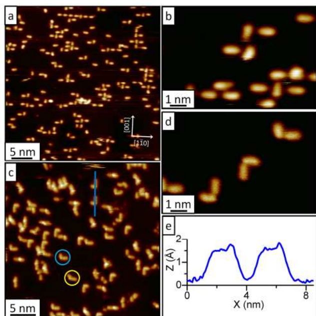
Fig 1. STM images of NEP deposited on Cu(110). (a) and (b), room temperature deposition, the observed features are the result of adsorption-induced fragmentation. (c) and (d), deposition at -130^{\circ}\text{C} , corresponding to intact molecules. The two main conformations are circled in (c). (e) Linescan over the blue line in (c) showing the methyl protrusions. All images were acquired at -196^{\circ}\text{C} .
