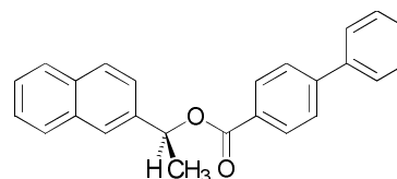
50 Scheme 1. ( S )-1-(2'-naphthyl)ethyl-(4-phenylbenzoate) (NEP)
