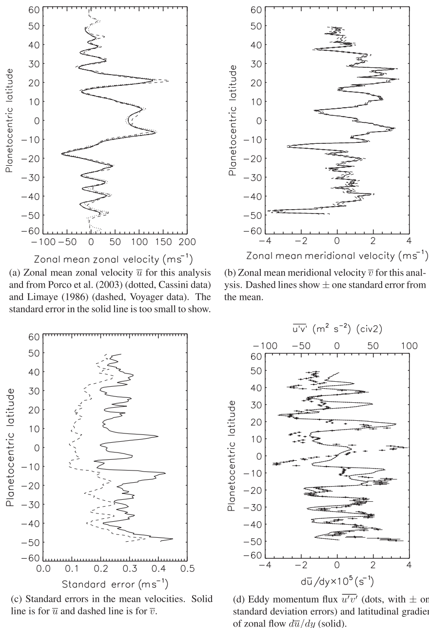
Fig. 4. Zonal mean diagnostics using data from all four days. Each profile uses all the filtered velocity vectors from all four days in latitude bins 0.5^\circ wide, without any weighting, rather than taking the average of the mosaiced fields, so any errors introduced by the mosaicing step are avoided.
