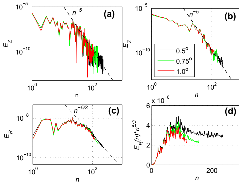
Fig. A.13. Zonal and residual kinetic energy spectra on Jupiter computed from our data with grid spacings of 1° (red), 0.75° (green), and 0.5° (black). (a) Three-day averaged zonal spectra E_z(n) ; the dashed line corresponds to Eq. (2a) with C_2 = 2 . (b) Spectra from (a) smoothed using a moving box algorithm with a five point stencil. (c) Same as (a) but for the residual spectra E_R(n) ; the dashed line corresponds to Eq. (2b). (d) Compensated residual spectra C_R = E_R(n)n^{5/3} derived from (c).
