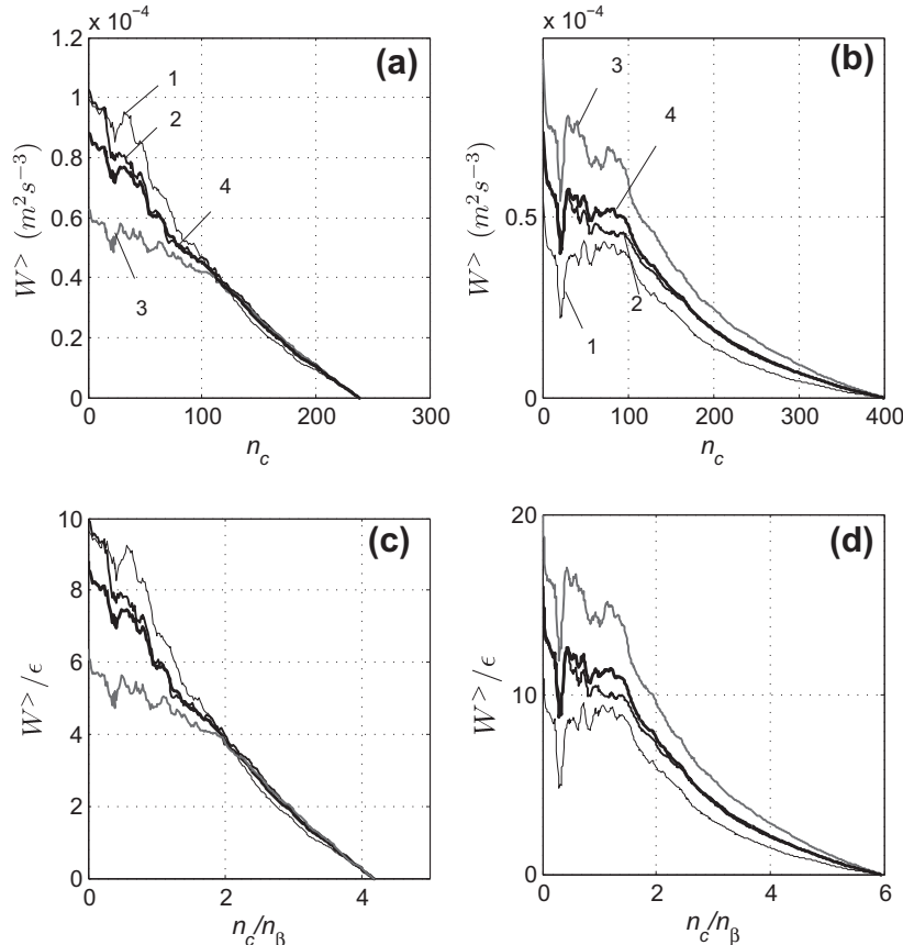
Fig. 11. Energy fluxes W^c (a and b) and normalized energy fluxes W^c/\epsilon (c and d) from the modes with n > n_c to the zonal flow. The three days as marked by numbers, with the line marked 4 being the three-day average. (a and c, left) show our data and (b and d, right) show CS data. In the normalized fluxes, the values of \epsilon are averaged over the three respective days.
