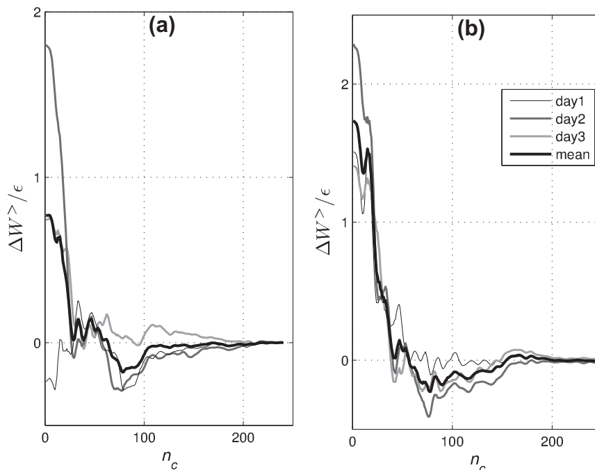
Fig. 12. The difference \Delta W^c between the energy fluxes with (W^c) and without (\widetilde{W}^c) the GRS. The values are normalized using the mean \epsilon for all three days. (a) Shows our data and (b) the CS data.
