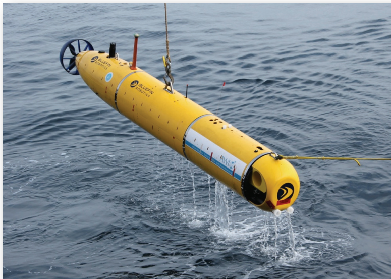
Fig. 3.2.1: Recovery of the AUV after a dive at HAUSGARTEN observatory
