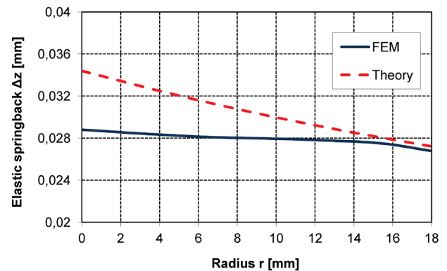
Figure 9 Elastic springback in axial direction
