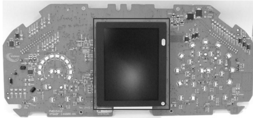
Figure 8: LCD: display of driver information (e.g. radio station)
