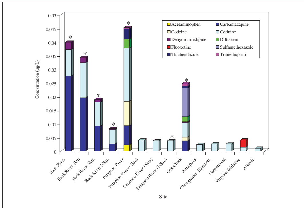
Figure 5. Concentration of compounds detected (excluding caffeine) in Chesapeake Bay water samples. *Erythromycin-H 2 O detected in these samples but not quantified.
