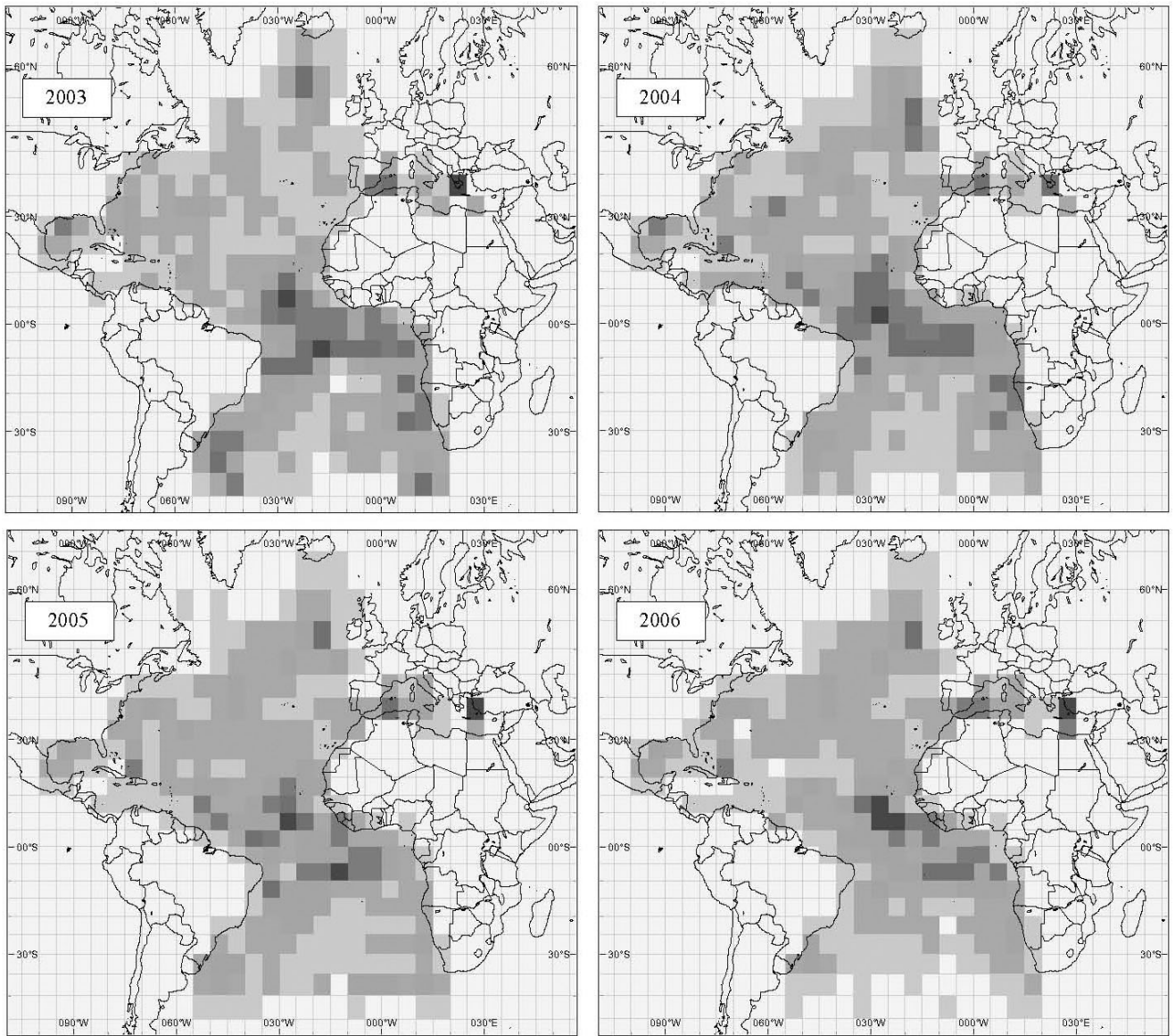
Figure 2.—Total ICCAT fisheries pelagic longline fishing effort annually 2003–06. Fishing effort is shown as shades of grey in 5 \times 5^\circ squares, with darker grey indicating higher effort.
