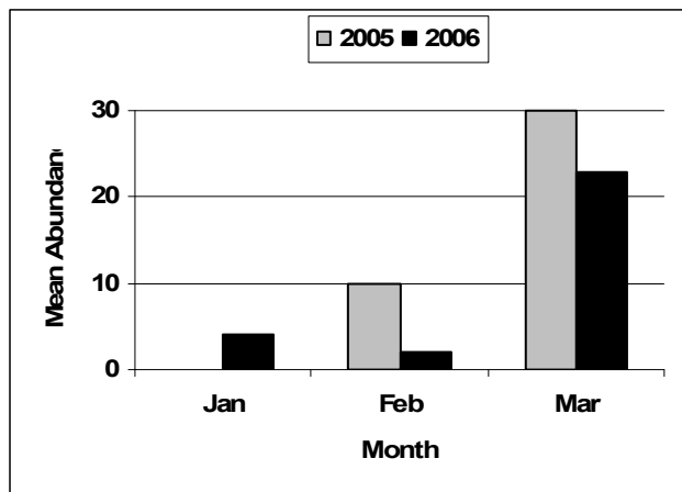
Figure 2. Mean abundance (individuals per dive) of Mycteroperca venenosa at aggregation.
