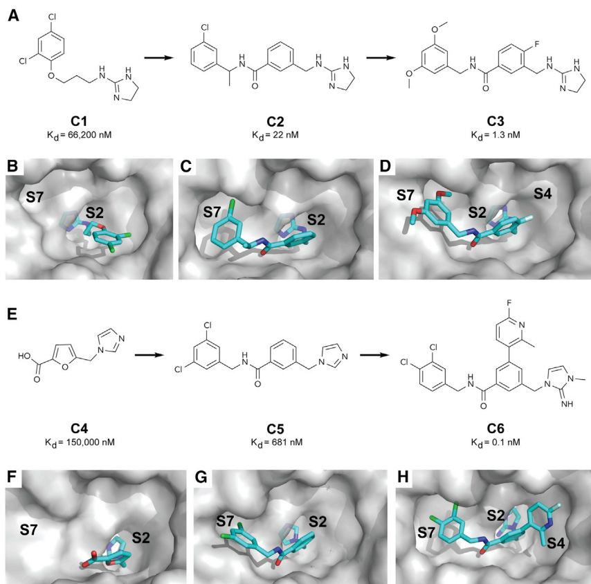
Figure 1. Discovery of Small Molecule WIN Site Inhibitors
