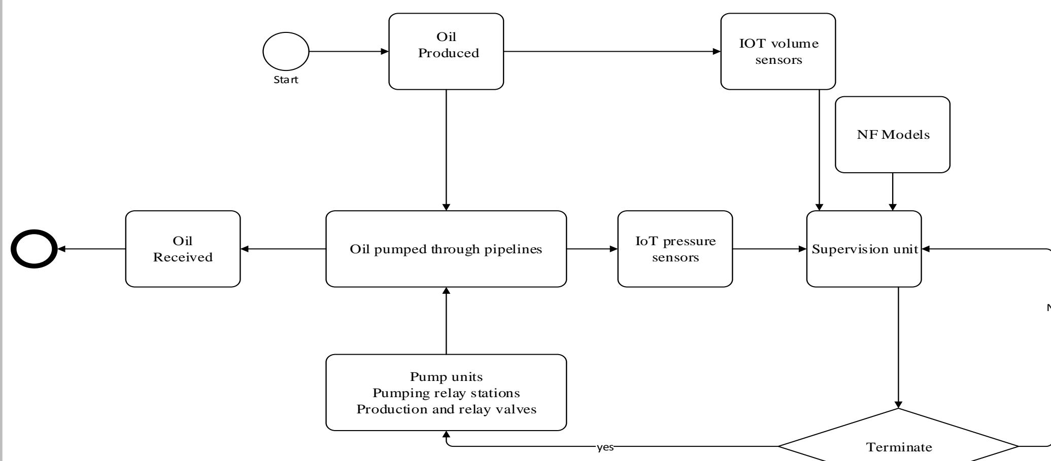
Fig. 1: Oil Pipeline Supervision System Flowchart
