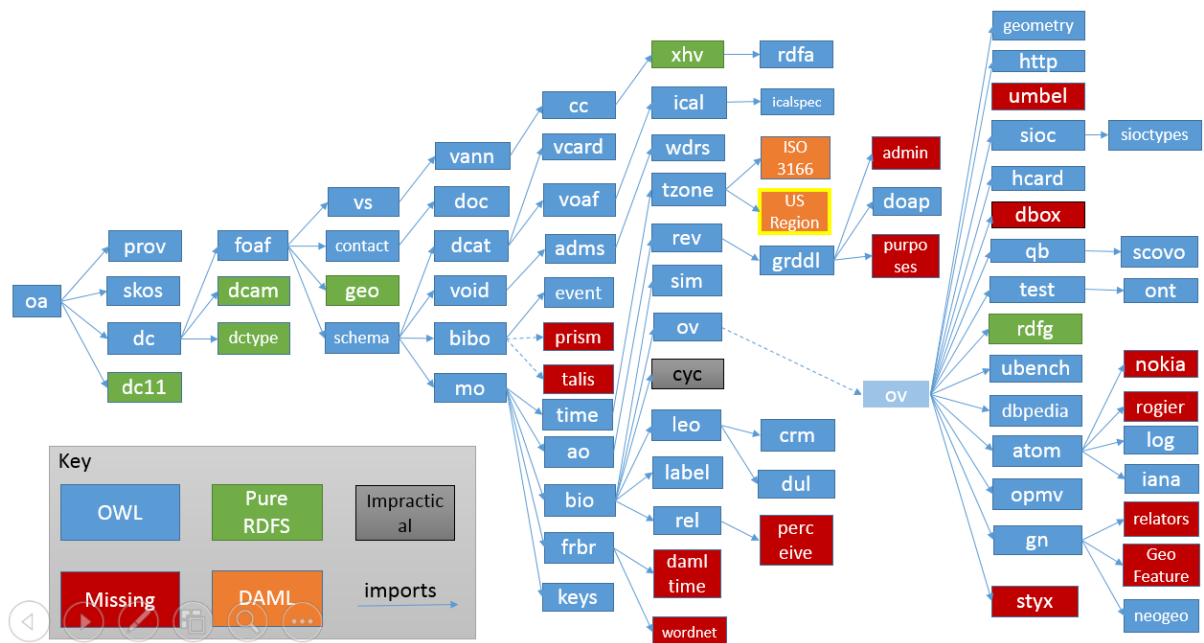
Figure 2 Open Annotation dependency tree of linked data vocabularies and ontologies
