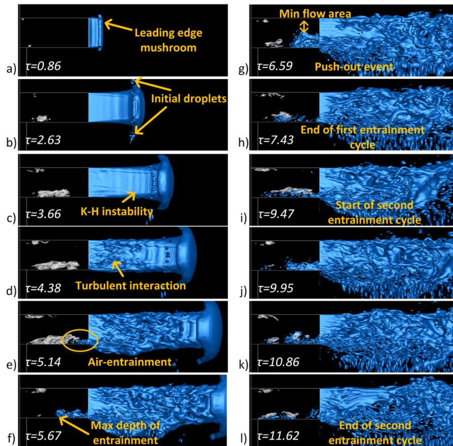
Figure 3: Evolution of in-nozzle cavitation and liquid jet at P_{inj} = 3 bar. Iso-surfaces of 50% vapour (white) and 95% gas (blue) volume fraction shown. The instances are chosen randomly over time to highlight the major events.
