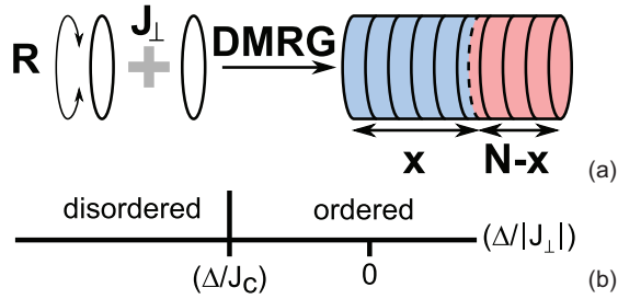
FIG. 1. (Color online) (a) An array of continuum chains of length R , with interchain coupling J_{\perp} . Each chain is a single site in our DMRG algorithm. (b) The phase diagram of coupled QICs.
