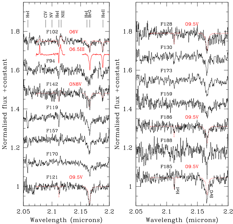
Fig. 3. K -band spectra of additional giant and main sequence cluster members; these have been rebinned to improve the S/N. Comparison spectra for O6 V (HD 5689), O6.5 III (HD 190864), O8 V (HD 13268) and O9.5 V (HD 37468) are overlotted in red and from Hanson et al. (2005).
