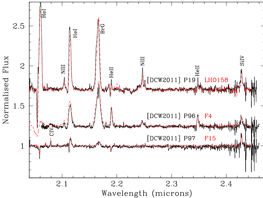
Fig. 6. K-band spectra of candidate runaways (black) compared to members of the Arches and Quintuplet (red; Clark et al. 2018a,b). [DCW2011] P96 and P97 show a close resemblance to WN7-8h and O6-7 Ia + stars within the Arches, while [DCW2011] P19 corresponds to the sole broad-lined WN9h star within the older Quintuplet.
