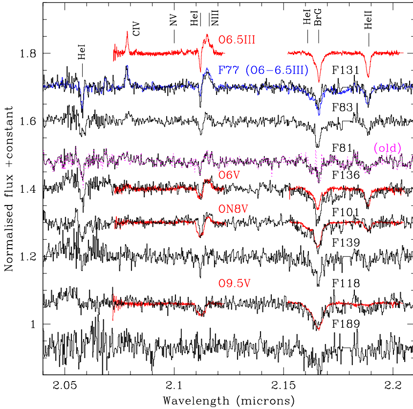
Fig. 2. K -band spectra of new or reclassified O6-O9.5 main sequence and giant stars within the Arches. A spectrum of the O6-6.5 III cluster member F77 is shown for comparison (blue) as are the template spectra for O6.5 III (HD 190864), O6 V (HD 5689), O8 V (HD 13268) and O9.5 V (HD 149757) stars (red; Hanson et al. 2005). Finally the spectrum of F81 from Paper I is reproduced (magenta) in order to illustrate the removal of spurious emission in the Br \gamma profile.
