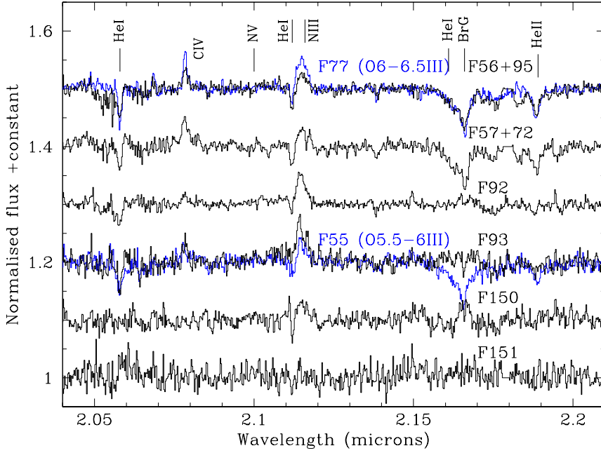
Fig. 5. K-band spectra of the blends of F56+F95 and F57+72 along with the anomalous sources F92, F93, F150 and F151 (see Sect. 3.1). Spectra of the cluster members F55 and F77 are overlaid in blue for comparison.
