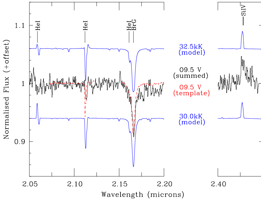
Fig. 4. K -band spectrum derived from the combination of individual spectra of candidate O9.5 V stars (black) plotted against template O9.5 V spectrum (HD 37468) and synthetic spectra for 32.5 kK and 30.0 kK O dwarfs (blue; Sect. 3.1). The region of the spectrum between 2.2 \mu m and 2.4 \mu m is both predicted and found to be featureless.
