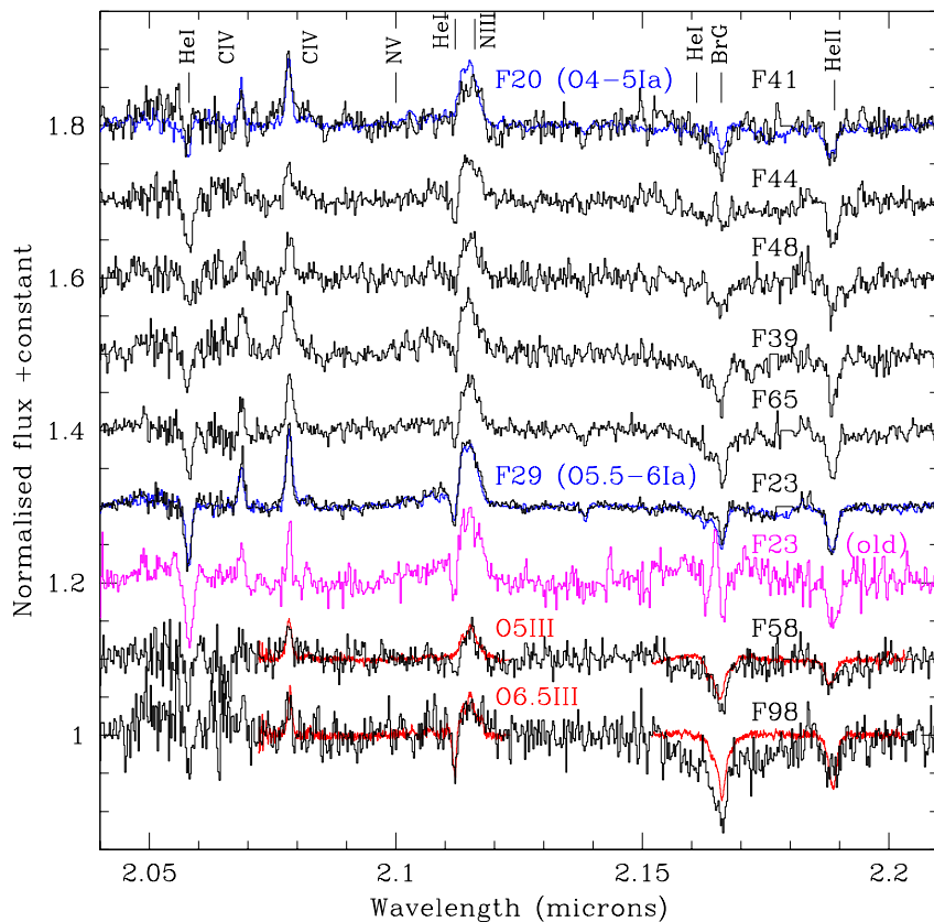
Fig. 1. K-band spectra of new or reclassified O4-6 giant and supergiant stars within the Arches. Spectra of supergiant cluster members F20 and F29 are shown for comparison (blue) as are the template spectra for O5 III (HD 15558) and O6.5 III (HD 190864) stars (red; Hanson et al. 2005). Finally the spectrum of F23 from Paper I is reproduced (magenta) in order to illustrate the increased S/N in the new data and also the removal of spurious emission in the Br \gamma profile of this particular star.
