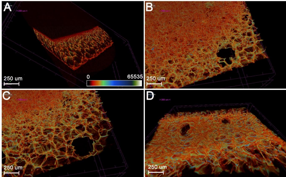
Figure 7. Micro CT image showing: an oblique cross-section through an unperforated, porous POSS-PCU scaffold (A), progressive longitudinal sections through a porous scaffold, laser perforated at intensity 6 (B and C) and 3 (D). Sections are taken from the volar (left) to dorsal (right) aspects.
