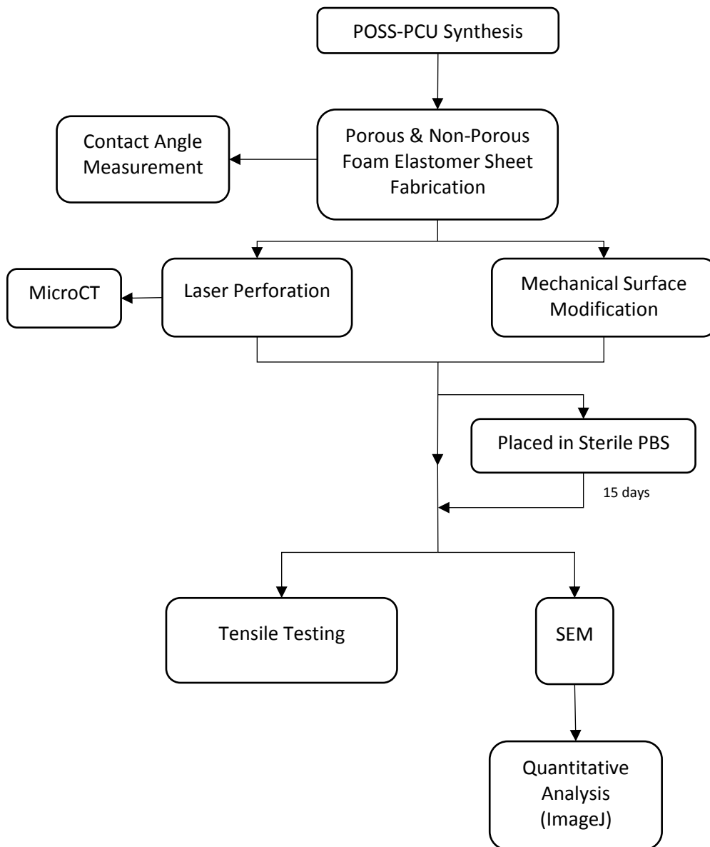
Figure 2. Flowchart summarising key steps and timelines of the characterisation experiments. Statistical analysis was also carried out.
