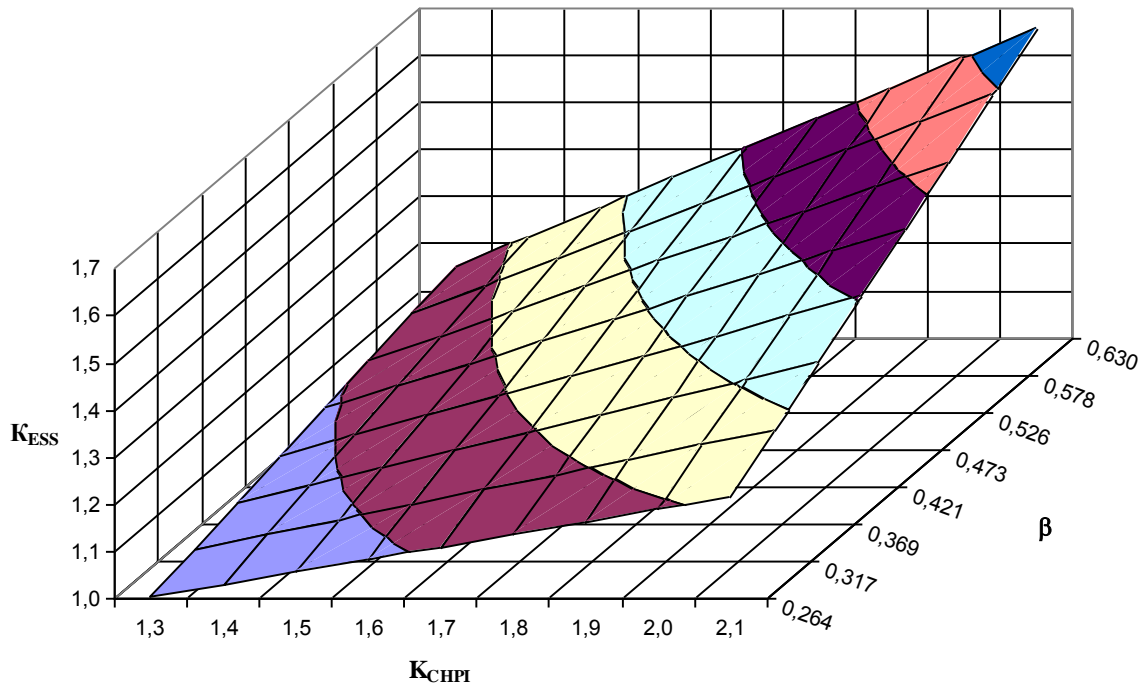
Fig. 2 – Area of high energy efficiency of ESS with CHPI of large power and peak fuel-fired boiler, on conditions of maximal efficiency of GPE and FB for heat supply systems
