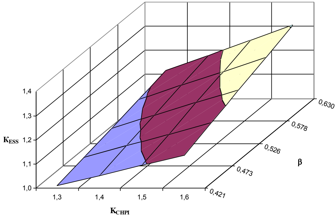
Fig. 1 – Area of high energy efficiency of ESS with CHPI of large power and peak fuel-fired boiler, on conditions of minimal efficiency of GPE and FB for heat supply systems
