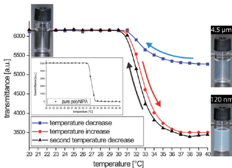
Fig. 4 Transmittance plots of the microparticle suspension recorded at decreasing temperature (A), followed by increasing temperature (B) and again decreasing temperature (C). The inset shows the transmittance plot of pure polyNIPAA. Next to the curves, photographs are shown of the corresponding liquids.
