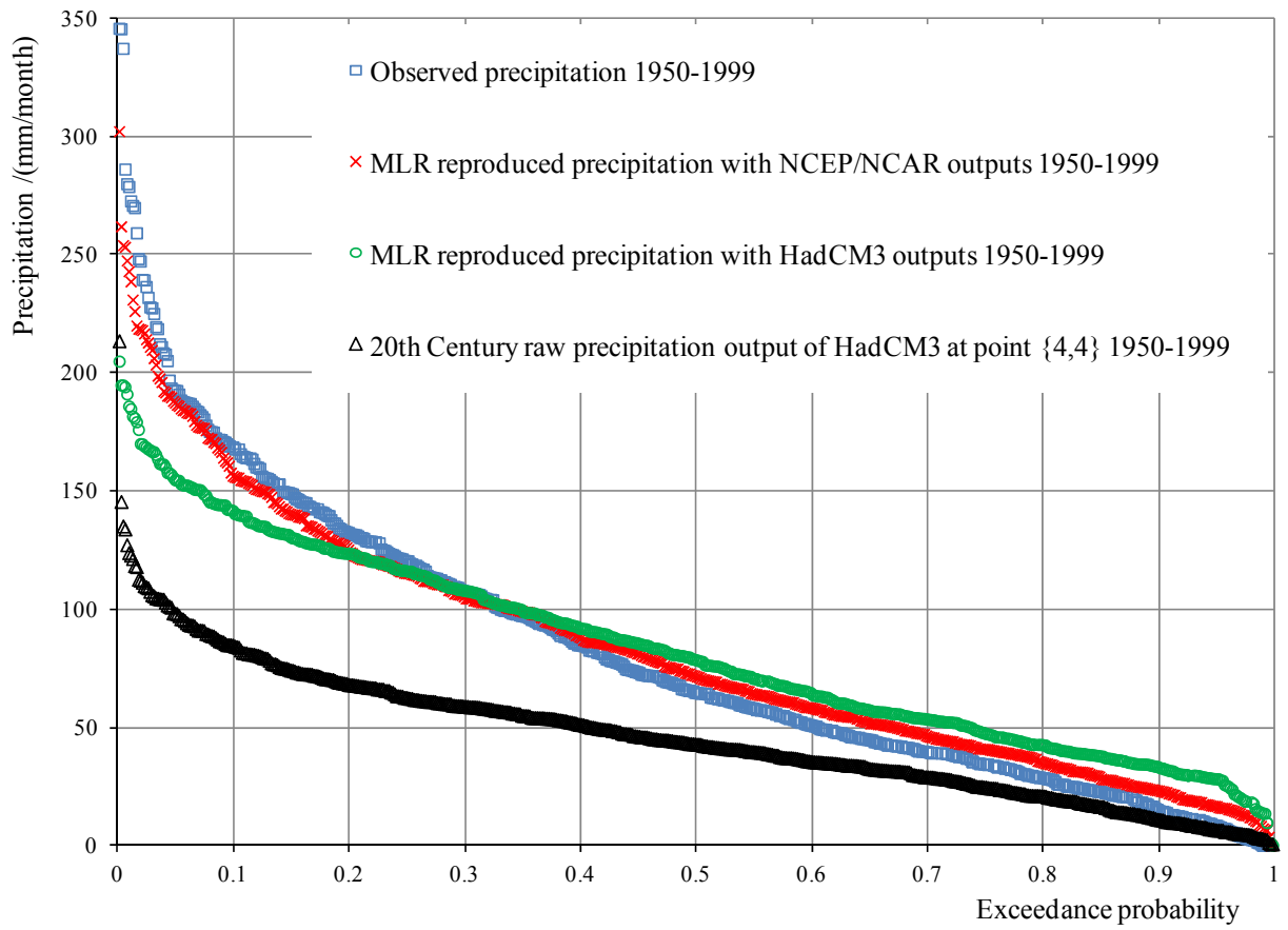
Figure 8 Precipitation probability exceedance curves (1950 to 1999)
