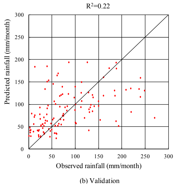
Figure 5 Scatter plots of observed and Model (HadCM3) reproduced monthly precipitation for calibration (1950-1989) and validation (1990-1999)
