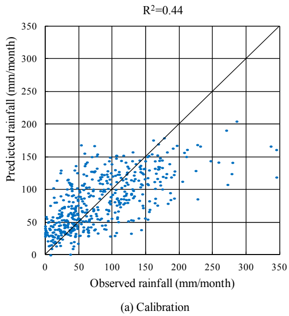
Figure 5 Scatter plots of observed and Model (HadCM3) reproduced monthly precipitation for calibration (1950-1989) and validation (1990-1999)
