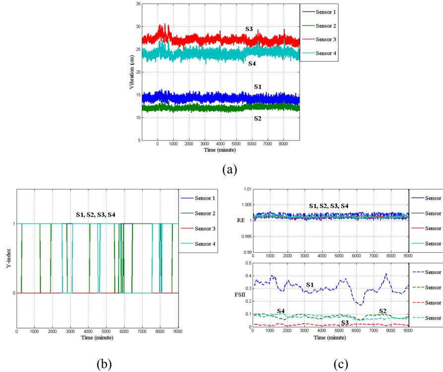
Fig. 7 Field Example 1: (a) Vibration measurements; (b) Y -index; (c) RE and FSII ( S =Sensor)
