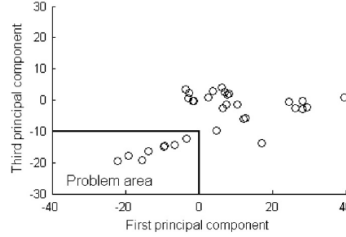
Fig. 1 First and third principal component plot for fault detection in aluminium electrolysis process [2]
