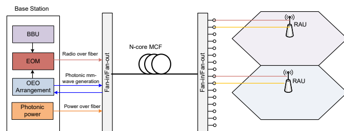
Fig. 1: Conceptual illustration of MCF-based mm-wave generation, RoF link and PoF. (BBU: Base band unit, RAU: Remote antenna unit, EOM: Electro-optic modulator, OEO: Optoelectronic oscillator)
