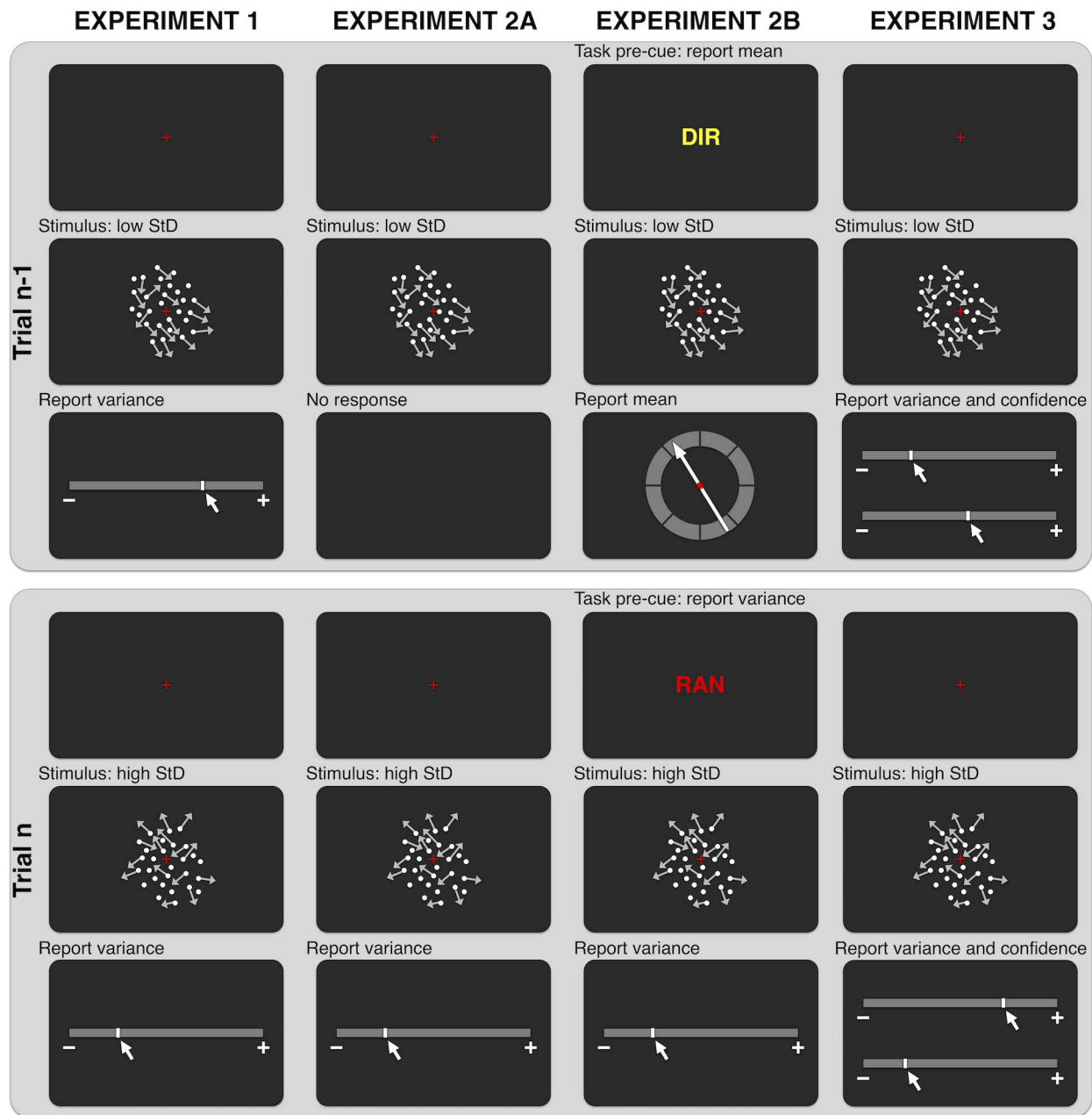
Figure 1. Experiments 1–3: Structure. In all experiments, each trial presented a random-dot kinematogram of a certain mean and variance (standard deviation, StD) in the motion trajectories of its component dots. In the example, Trials n - 1 and n have low and high StD values, respectively. Experiment 1 required variance (StD) reports for each trial, using a visual analogue scale. Experiment 2 interleaved two thirds of trials in which variance reports were required and one third in which either no response (Experiment 2A) or mean trajectory estimation (Experiment 2B) was required. In Experiment 2B the trial type was precued, so that the label “DIR” or “RAN” at the beginning of each trial indicated whether a mean or variance judgment was required for that trial. Experiment 3 required subjective confidence ratings following variance reports, using a similar visual analogue scale.
