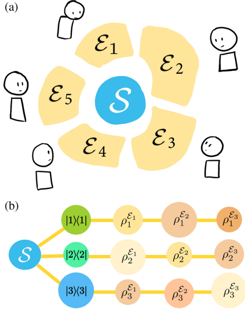
FIG. 1. Quantum Darwinism and spectrum broadcast structure. (a) Quantum Darwinism recognizes that the environment is made up of different fragments, for example, \mathcal{E} = \mathcal{E}_1 \otimes \mathcal{E}_2 \otimes \dots \otimes \mathcal{E}_5 . Different observers access the properties of the system by measuring different environment fragments. (b) A spectrum broadcast structure state can be viewed as the existence of different branches, where there are different, distinguishable states \{\rho_i^{\mathcal{E}_k}\}_i given different conditional system states.
