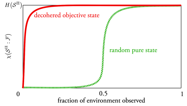
FIG. 2. Accessible classical information given by the Holevo information \chi(\mathcal{S}^\Pi:\mathcal{F}) about the system stored in different fractions of the environment. (Green dashed) For pure states picked out at random (through a Haar measure), the amount of accessible classical information and quantum discord are typically roughly the same. (Red solid) For a state that satisfies strong quantum Darwinism, such as the reduced GHZ state, \chi(\mathcal{S}^\Pi:\mathcal{F}) will be approximately equal to the system entropy H(\mathcal{S}) for small fractions of the environment, suggesting the existence of multiple copies of the information and hence redundancy [cf. analogous Fig. 2 in Zurek [4]].
