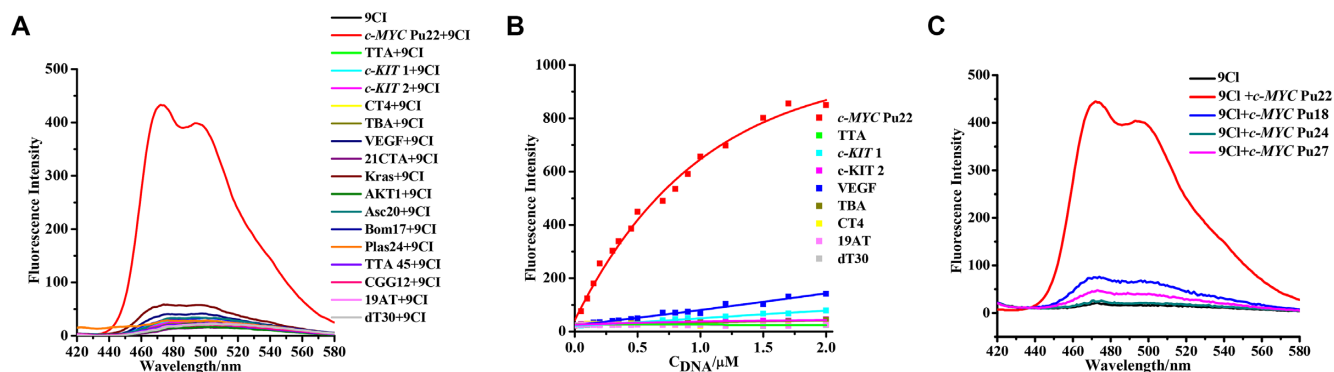
Figure 3. (A) Fluorescence emission spectra of 0.5 \mu\text{M} 9CI in the presence of various oligonucleotides (0.5 \mu\text{M} ), \lambda_{\text{ex}} = 405 \text{ nm} . Fluorescence emission of compound 9CI alone is shown in black. 0.5 \mu\text{M} oligonucleotide samples were in 10 mM \text{K}_2\text{HPO}_4/\text{KH}_2\text{PO}_4 buffer solution with 100 mM KCl at pH 7.0. (B) Fluorescence intensity enhancement of 0.5 \mu\text{M} 9CI against concentration of different DNA oligonucleotides. (C) Fluorescence intensity of 9CI in the presence of c-MYC Pu18, c-MYC Pu22, c-MYC Pu24 and c-MYC Pu27. Both 9CI and DNA are 0.5 \mu\text{M} . \lambda_{\text{ex}} = 405 \text{ nm} , \lambda_{\text{em}} = 472 \text{ nm} .
