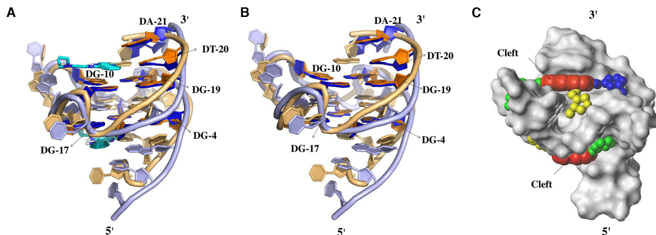
Figure 2. (A) Cartoon representation of superimposed c-MYC Pu22 G-quadruplex structures in apo state (brown, model 1 in the NMR structure, PDB 1xav) and with quindoline (purple, model 1 in the NMR structure, PDB 2l7v). The two quindoline molecules are shown in cyan. (B) Superimposed structures without ligands. (C) Connolly surface of c-MYC Pu22 G-quadruplex structure from PDB 2l7v. The red spheres highlight the central platform on top of 3' end G-quartet and at the bottom of 5' end G-quartet, while green, yellow and blue spheres represent the locations of grooves connecting to the central platform, respectively.
