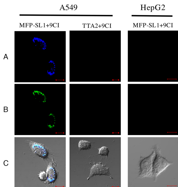
Figure 8. Confocal microscope images of the treated A549 cells and HepG2 cells at 405 nm excitation. A549 cells were incubated with SL1-M for 30 min at room temperature, and washed by 1 ml DPBS twice. Then, the cells were incubated with 500 nM MFP ( c-MYC Pu22-MFP/TTA-MFP) and 5 \mu M 9CI for 10 min. Fluorescence was collected after the cells were washed with DPBS three times again. (A) Fluorescence collected at 425–470 nm emission channel, (B) fluorescence collected at 500–545 nm emission channel, (C) merged image of (A) and (B) and bright field. Scale bar, 10 \mu m.
