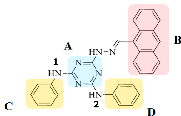
Scheme 1. Structure of 6-(2-(anthracen-9-ylmethylene) hydrazinyl)- N^2,N^4 -diphenyl-1,3,5-triazine-2,4-diamine (9CI) and its division into sub-structures. The triazine ring is labeled as A , and B represents the anthracene ring. C and D represent the phenyl rings. Nitrogen atoms connecting the triazine ring and the phenyl rings are labeled as 1 and 2 , respectively.
