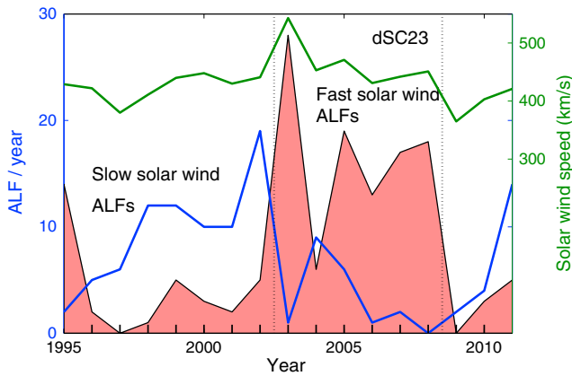
Figure 3. Yearly number of ALFs (left y axis) within slow (<400 km/s) solar wind (blue line) and within fast (≥600 km/s) solar wind (black line with pink shaded area) in 1995–2011. Yearly means of solar wind speed (right y axis) are denoted by a green line. Declining phase of SC23 and dSC23 is marked by dotted vertical lines.
