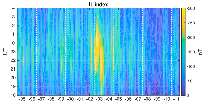
Figure 1. High-latitude geomagnetic activity based on IL, the westward electrojet index in Scandinavian sector in 1995–2011. Amplitude of IL index (in nT) is color-coded such that the largest monthly disturbances are shown by yellow and smallest by blue.
