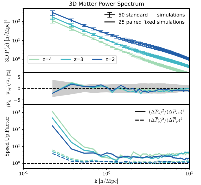
Figure 1. Matter power spectrum measured at z = 2, 3, and 4 . The top panel shows the mean power spectrum in the two sets of simulations, the standard simulations, \bar{P}_S , with the 1\sigma uncertainty on the mean, and the paired–fixed simulations, \bar{P}_{\text{PF}} ; the means are indistinguishable. The middle panel shows the fractional difference between the mean power measured in the two sets of simulations, with a shaded region showing the expected 1\sigma uncertainty on that difference which is given by Equation (10). Across all scales, there is no evidence for bias in the estimate of the paired–fixed simulations relative to the traditional simulations. The bottom panel shows the ratio between the uncertainty on the mean of the standard and paired–fixed simulations, (\Delta\bar{P}_S)^2/(\Delta\bar{P}_{\text{PF}})^2 , with dashed lines showing instead the effect of fixing without pairs (\Delta\bar{P}_S)^2/(\Delta\bar{P}_F)^2 . These ratios summarize how fast the paired–fixed (or fixed) simulations converge on the mean power spectrum relative to the standard simulations. As a typical example of improvement, for wavenumbers k = 0.25 h\text{Mpc}^{-1} and 2 h\text{Mpc}^{-1} at z = 3 , we find estimates of the matter power spectra converge 390 and 2.0 times faster in the paired–fixed simulations compared with the standard simulations.
