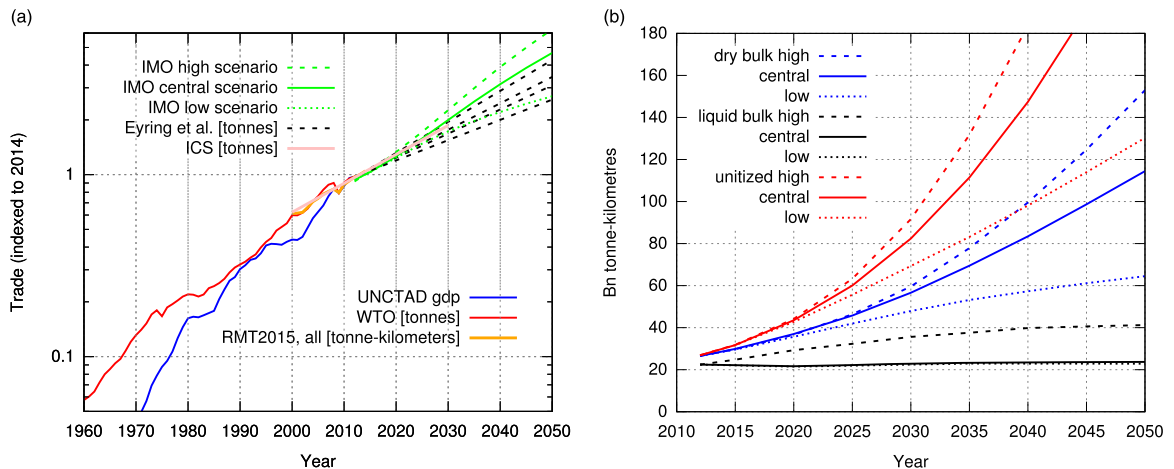
Figure 1. Scenarios of future demand for sea transport. Left: High, central, and low demand scenarios (Smith, Jalkanen et al., 2015); historical data of transport demand in tonne-kilometres (UNCTAD, 2015), international trade in tonnes (data from (WTO, 2015)), and GDP (data: UNCTAD, 2016, gross domestic product: total, constant (2005) prices, annual, 1970–2014); a market forecast of transport demand in tonne-kilometres [data: International Chamber of Shipping: Shipping, World Trade and the Reduction of CO 2 Emissions], and a suite of future scenarios of transport demand in tonnes from the climate change literature (Eyring et al., 2005). Right: Demand for dry bulk, wet bulk, and unitized cargo in high, central, and low growth scenarios (Smith, Jalkanen et al., 2015).
