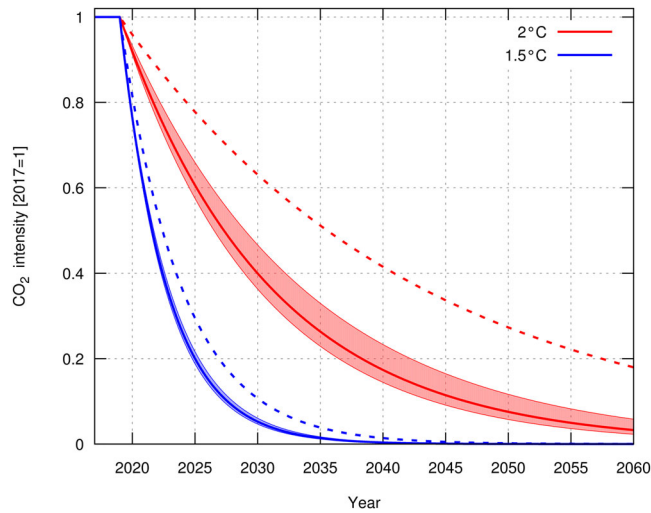
Figure 2. Average CO 2 intensity, reducing by constant year-on-year factor, from 2020 onwards, in 2°C scenario (less steep) and 1.5°C (steeper reductions). Shaded areas cover range from low to high demand growth scenario, with central demand scenarios shown as solid lines. Dotted lines show case of zero demand growth.
