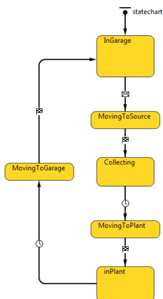
Fig. 2. Example state chart of transportation (truck/tanker) agent.
