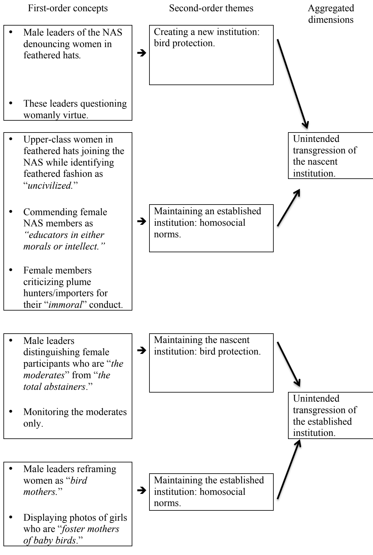
Figure 1. Data Structure.
