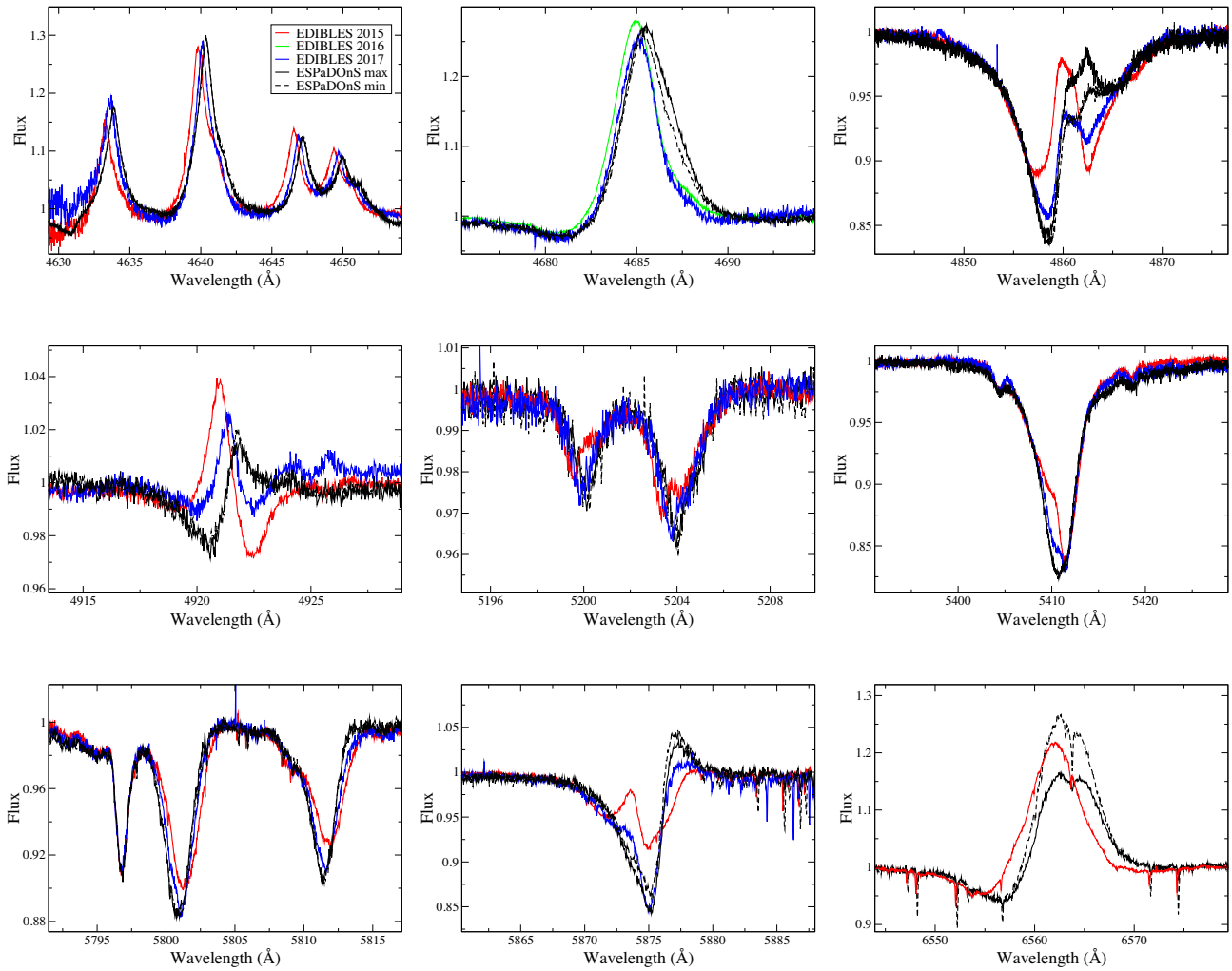
Figure 2. The black (solid and dashed) profiles show the range of variability of each spectral line in the ESPdOnS data set of Wade et al. (2012). The red, green, and blue profiles show the EDIBLES observations obtained in 2015 (JD 2457251), 2016 (JD 2457644), and 2017 (JD 2457867), respectively. Spectra are in the heliocentric reference frame and have not been corrected for telluric absorption.
