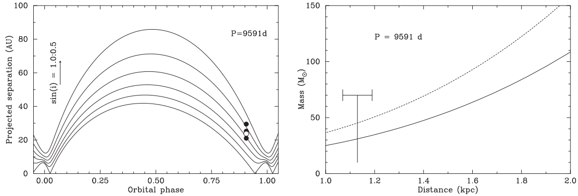
Figure 5. Left – Projected separation of the components of HD 148937 assuming the longer period ( P = 9591 d) orbital solution. The curves correspond to inclinations \sin i = 1.0, 0.9, 0.8\dots (from the bottom up). The filled circles are the separation for assumed distances of 1.0, 1.2, and 1.4 kpc (bottom to top). The open circle represents the Gaia DR2 distance, for reference. Right – Constraint that the single SMASH + observation provides on masses as a function of distance. The two curves correspond to M_1 and M_2 . The Gaia DR2 distance is indicated by the vertical line. We remind the reader that the Gaia distance may be systematically affected by the presence of the close interferometric companion.
