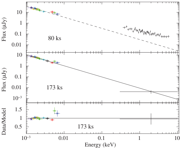
Fig. 2. Spectral Energy Distributions (SEDs) of GRB 130831A at 80 ks (top) and 173 ks (2 days) after the trigger (bottom). We plot on the 173 ks SED the best-fit model, a power-law of index \beta_{OX} = 1.03 . We rescale this model by (173/80)^{1.59} , where 1.59 is the temporal decay slope, and draw it on the 80 ks SED (dashed line). Such an extrapolation predicts the optical, but clearly underestimates the X-ray emission, which must be due to a component absent at 173 ks.
