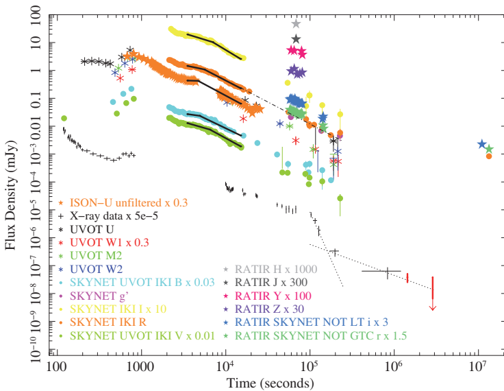
Fig. 1. GRB 130831A UVOIR and X-ray light-curves. XRT and Chandra data points are black and red respectively. Data between 230 ks and 6000 ks are not shown because they are contaminated by SN 2013fu, associated with this GRB. The reader is referred to Cano et al. (2014) for a complete study of the supernova. Data points at \simeq 10^7 s are due to the host galaxy. On the optical light-curves, we show the best fit model between 3.5 and 15 ks (see De Pasquale et al. 2016 for more details). On the R band and X-ray light-curves, we plot the best-fit power-law model (dashed and dotted lines) between 15 and 230 ks. More specifically, the X-ray band model shows two power-laws that contribute to the flux.
