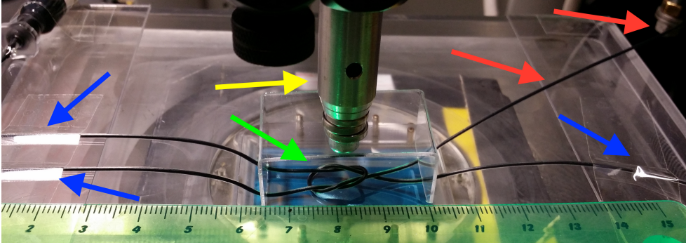
FIG. 8. Experimental setup for dynamic, stop-motion phantom: The two polythene tubes are immersed in a bath of intralipid solution placed on the FP sensor plane (green arrow). Three of the tube ends are fixated (blue arrows) while one is tied to a motor shaft (red arrows). The excitation laser (yellow arrow) is illuminating from the top.
