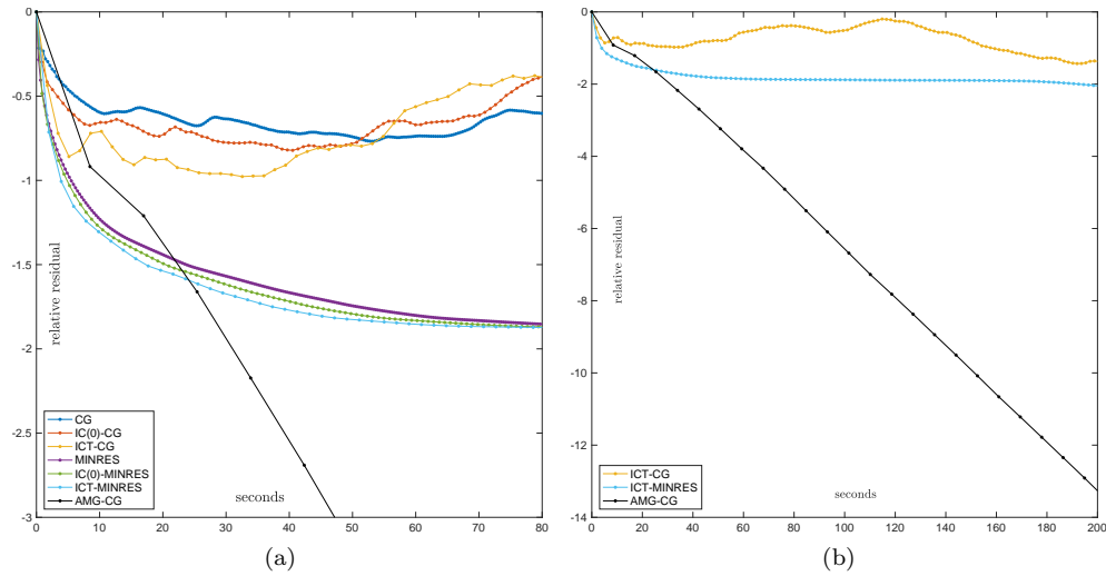
FIG. 12. (a) Comparison between different iterative methods and pre-conditioners to solve (4.17) (see Section 5.3 for the details of the set-up). The vertical axis shows the relative residual while the horizontal axis shows the computation time on a single CPU core averaged over 10 repetitions. (b) The same plot with only a subset of the solvers and expanded axis.
