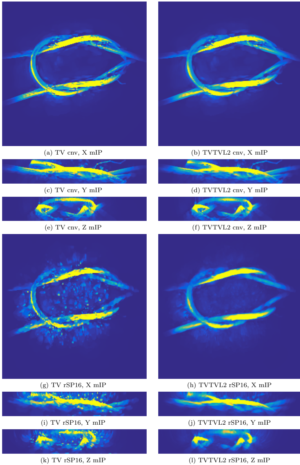
FIG. 9. Snapshots at t = 23 of the reconstructed pressure p for full ( cvt ) and sub-sampled ( rSP-16 ) experimental data.
