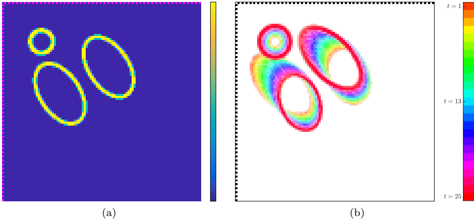
FIG. 3. The 2D numerical phantom. (a): A snapshot at t = 13 and the corresponding color bar. The sensor locations are shown as pink pixels (left and top edge). (b) A visualization of all T = 25 frames as a color-coded RGB overlay. The color bar displays which colors are assigned to which time frame, the sensor pixels are shown as black pixels.
