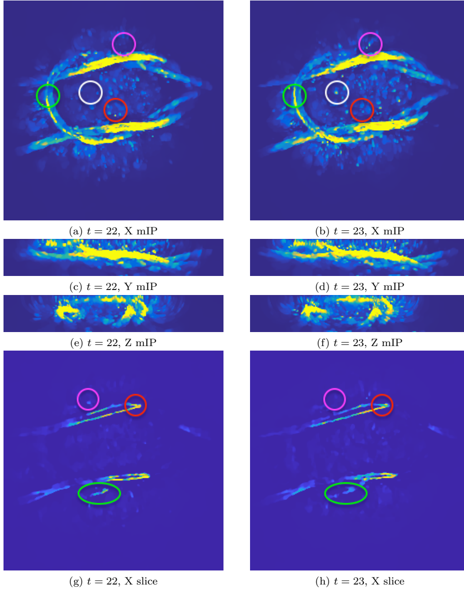
FIG. 2. Limitations of applying frame-by-frame image reconstruction (2.5) to a dynamic PAT data set (details given in Section 5.2) when using a high sub-sampling factor M_{\text{sub}} = 16 : Figures in the left and right column show maximum intensity projections (mIP) along different directions ((a)-(f)) and slice view visualizations ((g)-(h)) of the results p_{22} and p_{23} , respectively. One can easily see that image artefacts are not correlated between the two subsequent time frames (same coloured circles in left and right images highlight examples) while the target's motion is.
