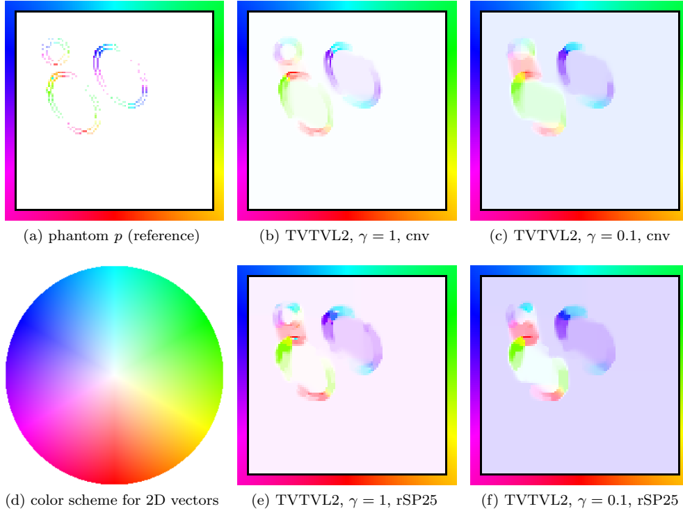
FIG. 7. Illustration of the reconstructed motion fields v for the results shown in Figure 5. First, each vector field is rescaled such that \max_i \|v_i\|_2 = 1 . Then, each pixel i is coloured by mapping direction and norm of v_i to the color scheme displayed in (d). To further ease the visualization, a coloured frame was added to each motion image to depict the colors corresponding to a vector pointing from the middle of the image to the pixels of the frame. The motion field for the phantom (a) was computed by solving (4.5b) with the true p as input and \gamma = 1, \beta = 10^{-6} .
