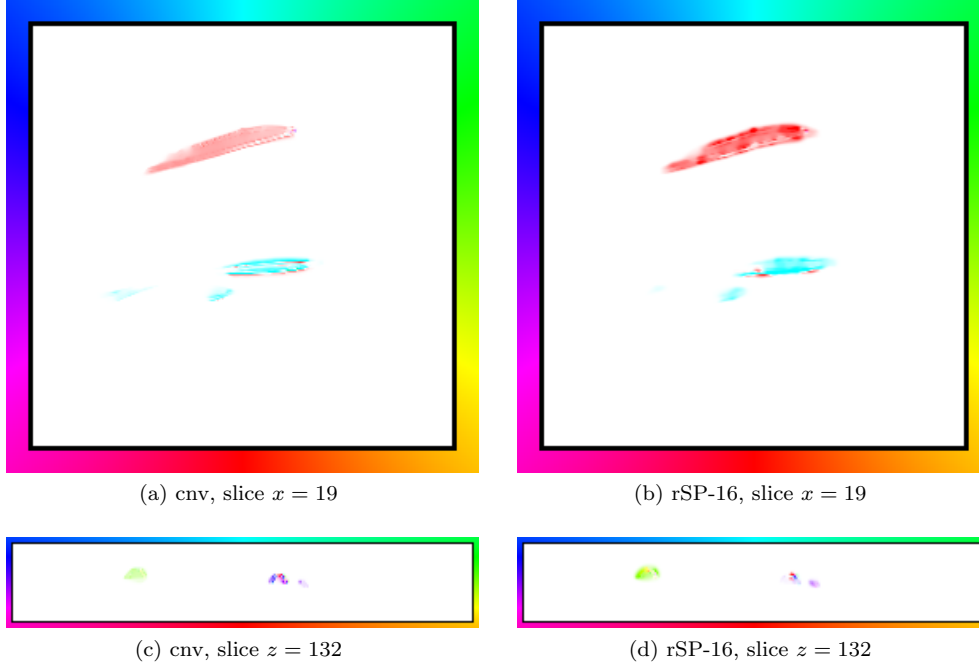
FIG. 10. Snapshots of the non-translational part of the motion field v^{\text{NT}} = v - N^{-1} \sum_i v_i reconstructed by the TVTVL2 method for full (cnv) and sub-sampled (rSP-16) experimental data between frames t = 22 and t = 23 . For each image, a single slice along a particular dimension was extracted and only the components of the vector field in the remaining two dimensions is depicted here. The resulting 2D vector field is color-coded in the same way as in Figure 7.
