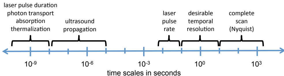
FIG. 1. Sketch of the relevant time scales in high resolution 4D PAT with sequential acquisition: PAT is particularly suited to image dynamic processes in living tissue that are related to blood circulation. For this, one would ideally like to obtain a temporal resolution close to the heart beat ( \sim 1 s for humans, \sim 0.1 s for mice). As the processes that contribute to a single PA signal take place within nanoseconds to microseconds, the main temporal limitation of sequential acquisition systems is given by the excitation laser pulse rate. Lasers with sufficiently high pulse energies are currently limited to \sim 200 Hz, which typically leads to longer acquisition times for a complete scan than what is desired. For instance, scanning 20 000 locations with a 20Hz laser takes 1000s while using a 200Hz laser in combination with a multi-beam read-out system as described in [41] takes 12.5s. In the latter case, applying compressed sensing with a sufficiently high sub-sampling factor would yield the desired temporal resolution.
