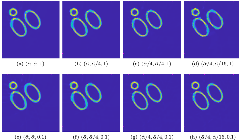
FIG. 6. Snapshots at t = 13 of the results of the TVTVL2 image reconstruction (3.5) for sub-sampled ( rSP-25 ) data for different combinations of (\alpha, \beta, \gamma) . Here, \hat{\alpha} corresponds to the value of the regularization parameter used for the TV-fbf reconstructions in Figure 4.
