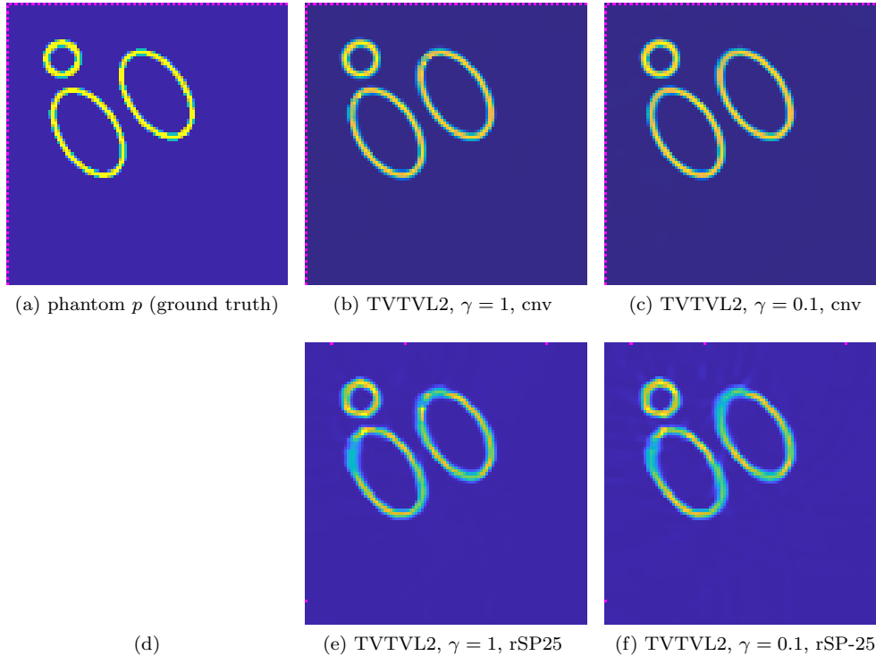
FIG. 5. Snapshots at t = 13 of the results of the TVTVL2 image reconstruction (3.5) for full (cnv) and sub-sampled (rSP-25) data. The parameters \alpha and \beta were set to the corresponding value of the \alpha used for the TV-fbf reconstructions in Figure 4 and \gamma was set to 1 or 0.1.
