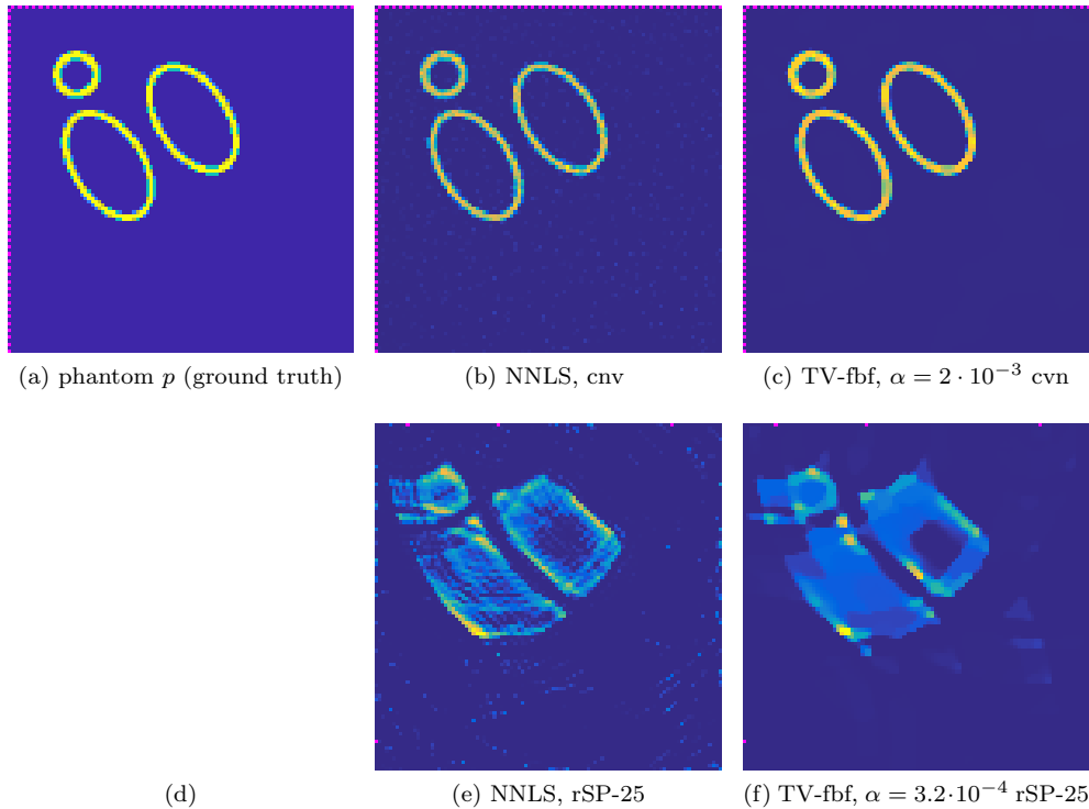
FIG. 4. Snapshots at t = 13 of the results of frame-by-frame image reconstruction methods (2.5) for full (cvn) and sub-sampled (rSP-25) data.
