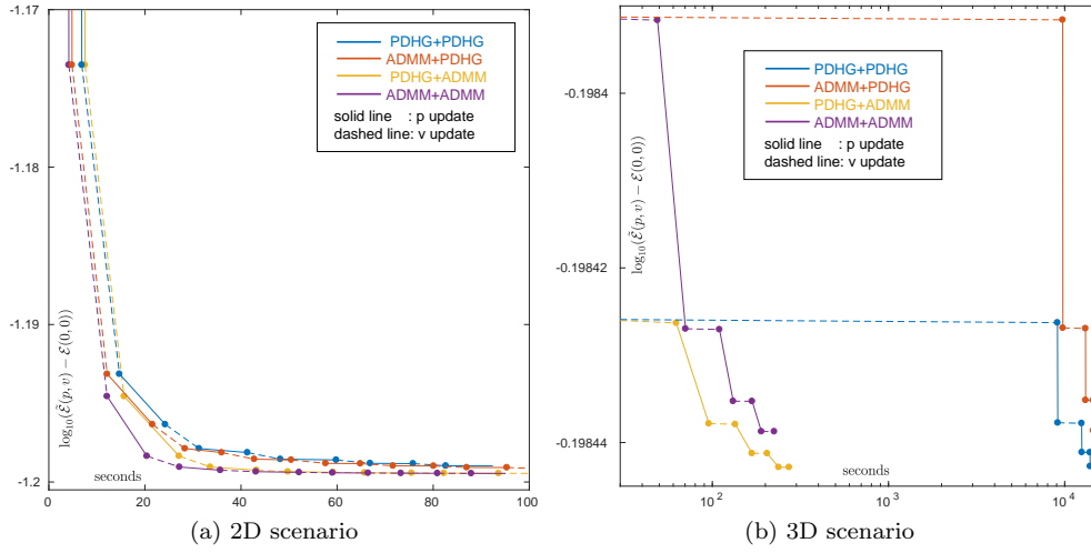
FIG. 11. Comparison of different methods to solve the bi-convex optimization problem (4.4) via ACS for (a) the 2D example described in Section 5.1 and (b) T = 10 frames of the 3D scenario described in Section 5.2. The plots display the decay in energy \tilde{\mathcal{E}}(p, v) relative to the initialization with p = 0, v = 0 vs computational time in seconds (in logarithmic scale in (b)). Solid parts of the line plots correspond to the p update (4.5a) and dashed parts to the v update (4.5b). A total of 4 ACS alternations is displayed. "ADMM-PDHG" refers to using ADMM for p update and PDHG for the v update.
