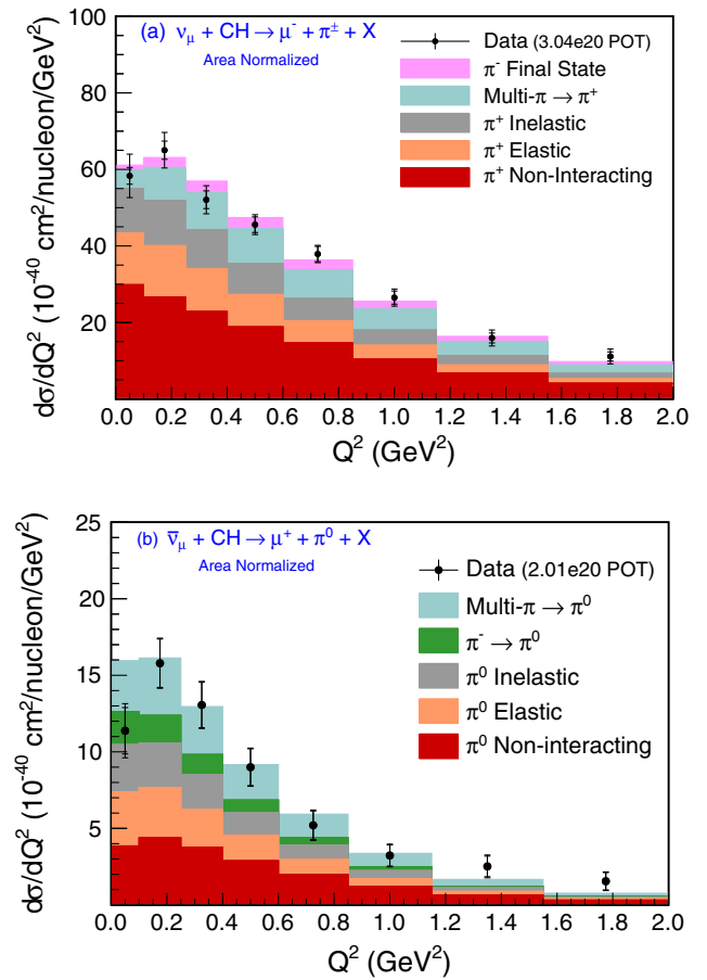
FIG. 14. Breakout of pion FSI processes within GENIE cross-section predictions for the two analysis samples. Stacked histograms (top to bottom) show contributions from \pi^- (for the charged pion sample), multiple-pion production with absorption, charge exchange (for the \pi^0 sample), inelastic scattering, elastic scattering, and no interaction. The full simulation, shown area-normalized to the data, reproduces the shape of data d\sigma/dQ^2 without ascribing Q^2 -dependence to pion FSI.
