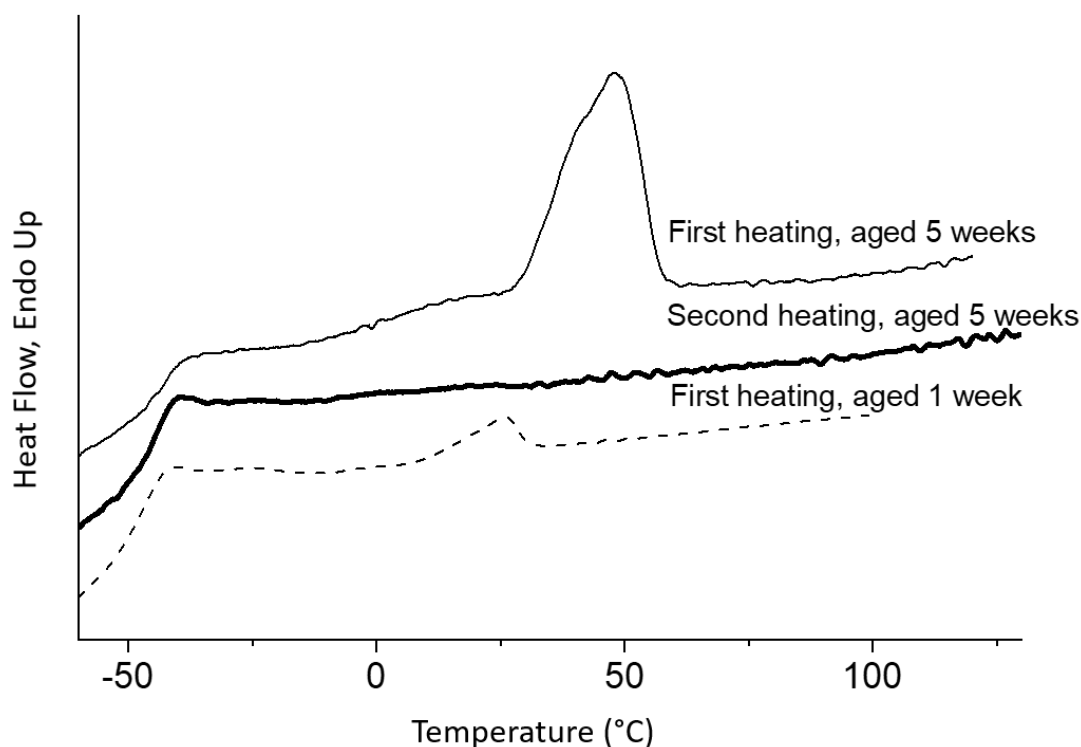
Fig. 3. DSC thermograms of P(3HO-3HD-3HDD) aged for 1 and 5 weeks at room temperature.
