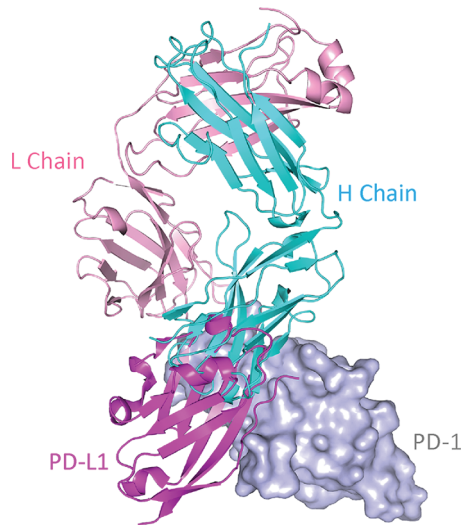
Figure 3. Crystal structure of the IBI308 (Sintilimab) Fab-PD-L1-PD-1 complex. The light (L) and heavy (H) chains of Sintilimab Fab are shown in salmon and cyan, respectively. PD-L1 is in pink and PD-1 is in light blue (surface representation). The structure suggests that IBI308 can efficiently block PD-1/PD-L1 and PD-1/PD-L2 interactions (PD-L1 and PL-L2 binding sites on PD-1 are mostly overlapped). In addition, the binding epitope of IBI308 is distinct from that of Pembrolizumab and Nivolumab.
