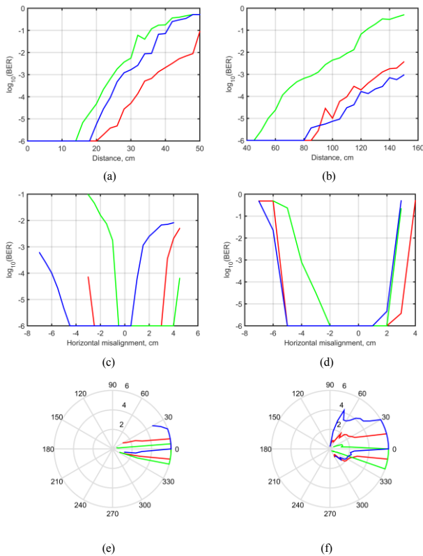
Figure 5 Experimental results of the WDM RGB LED showing: (a) BER as a function of distance between the Tx and Rx w/o lens, (b) with a lens, (c) horizontal displacement w/o lens, (d) with lens, (e) angular misalignment w/o lens, and (f) with lens.
