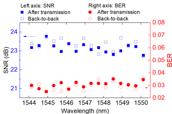
Fig. 5 Measured SNR (square marker) and BER (circle marker) both back-to-back (open marker) and after transmission (closed maker) through the 270-m HC-ARF fiber link.
