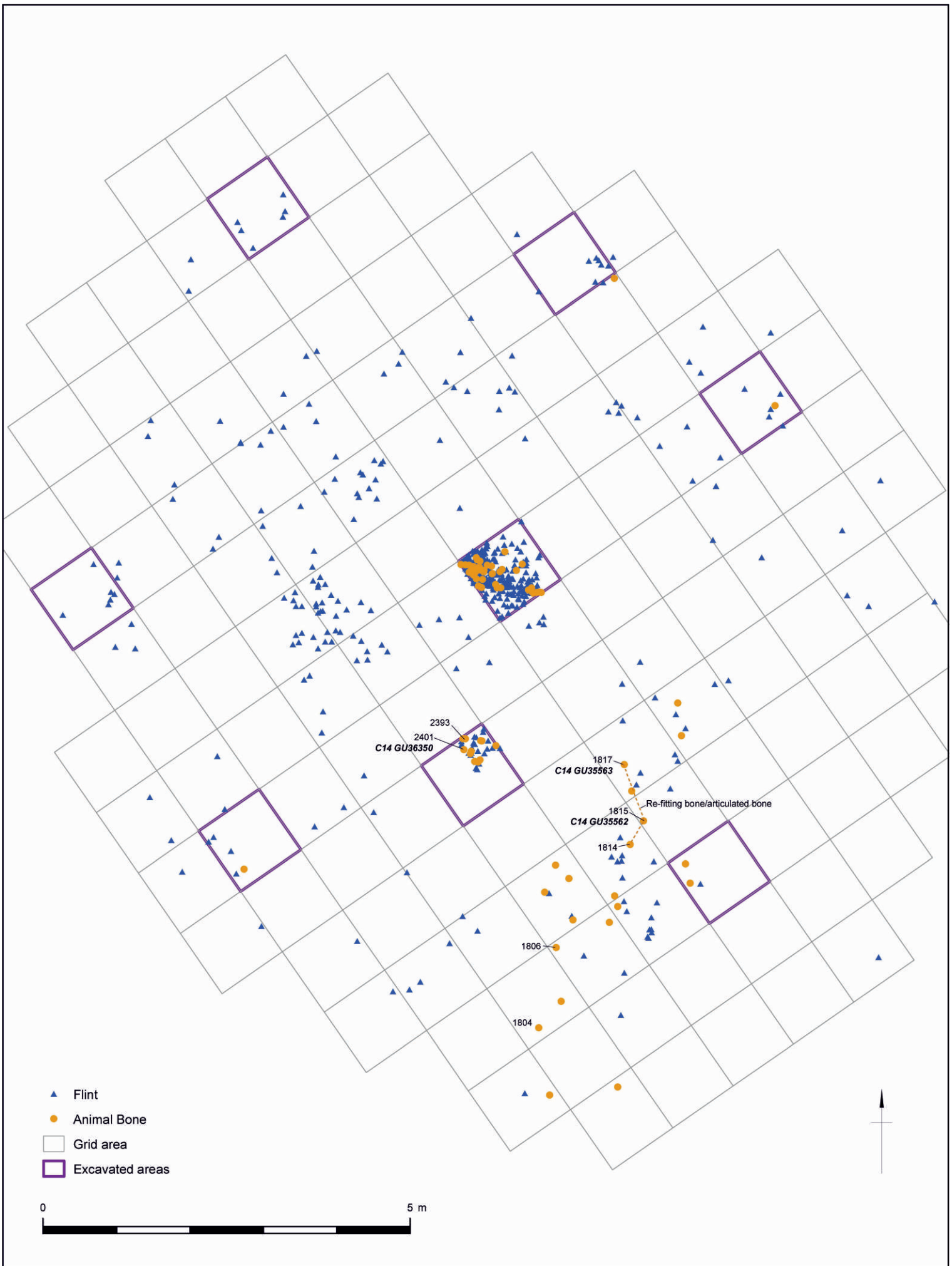
Distribution of all recorded flint and animal bone, and the location of the C14 samples and the articulating horse bone
