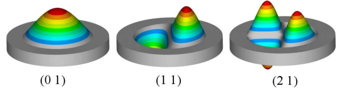
Fig. 13. Modal shapes the circular membrane with mode indexes (n_0, n_1) . The color scale, from light gray to red, is proportional to the absolute displacement from the equilibrium position.
