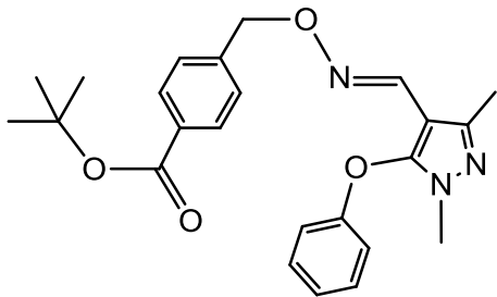
Fenpyroximate (2)
