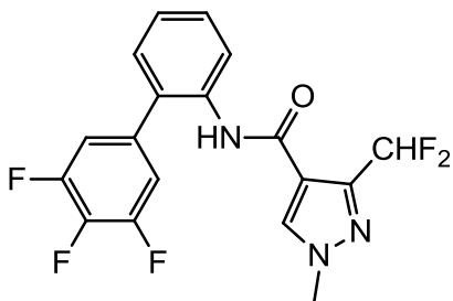
Fluxapyroxad (5)
