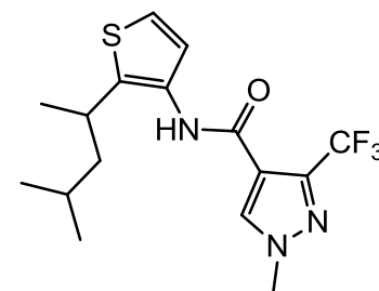
Penthiopyrad (8)
