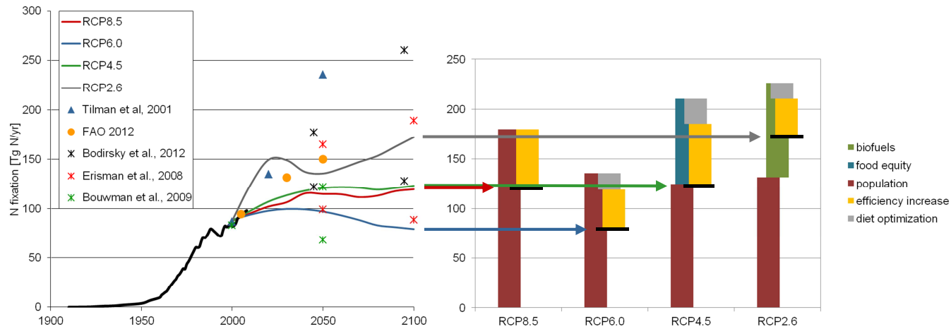
Fig. 2: Global agricultural demand for industrial N fixation (Tg N/yr), projected till 2100. Lines in the left panel reflect trends attributed in this paper to the respective RCP scenarios, while dots and asterisks show other assessments. The asterisks express the ranges (maximum and minimum) out of several scenarios based on storylines, with Erisman et al. (2008) using a methodology very similar to the one applied here for RCPs. Global population numbers used for 2100 are 12.4 billion, 9.34 billion, 8.6 billion and 9.06 billion (RCP8.5, RCP6.0, RCP4.5 and RCP2.6, respectively).
