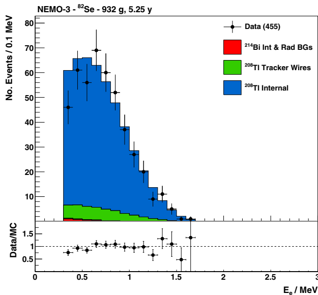
Fig. 5 Energy spectrum of electrons selected in the 1e2 \gamma channel, which contains an electron and two \gamma -rays. The channel is designed to allow a measurement of the source foil contamination with ^{208}\text{Tl} . Data are compared to the MC prediction, which is dominated by internal ^{208}\text{Tl} contamination with a small contribution from ^{208}\text{Tl} in the tracker wires
