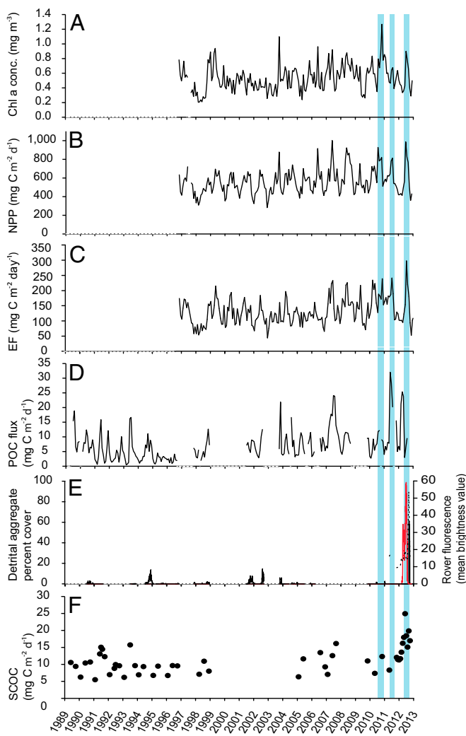
Fig. 1. Long time-series measurements of surface-ocean and abyssal processes from July 1989 through November 2012 at Station M in the northeast Pacific Ocean on a monthly basis. Blue bars highlight the timing of peaks in NPP from 2010 to 2012. Dashed lines on x axes indicate data gaps longer than 1 mo. (A) Chlorophyll a concentration within 100-km-radius circle around Station M. (B) Net primary production within 100-km-radius circle around Station M. (C) Satellite estimated EF in a 100-km-radius circle around Station M, calculated for a nominal depth of 100 m. (Dataset S1). (D) POC flux. (E) Phytodetrital (black) and salp (red) aggregate percent cover on the sea floor (daily averages). Benthic Rover fluorescence images relative brightness value (dashed line). (F) Monthly averages of SCOC measured seasonally from 1989 until 2011 and daily from 2011 through 2012 (oxygen consumption has been converted to milligrams of carbon assuming a respiratory quotient of 0.85).
