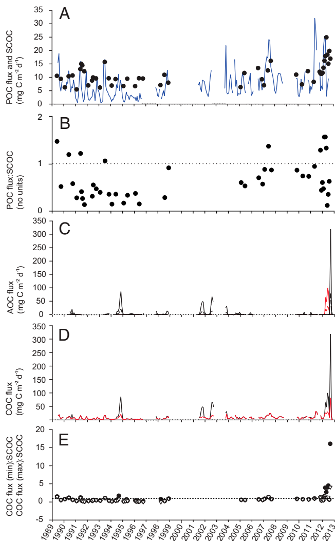
Fig. 2. Comparisons of food supply as POC and sea floor AOC with food utilization by the benthic community (SCOC) at Station M from July 1989 through November 2012. Dashed lines on x axes indicate data gaps exceeding 1 mo. (A) POC flux (line) and SCOC (dots). (B) Ratio of POC flux to SCOC. (C) Monthly estimated organic carbon flux of detrital aggregates (AOC) on the seafloor expressed in milligrams of C\ m^{-2}\ d^{-1} . Phytodetrital AOC flux (black lines) minimum (dashed line) and maximum (solid line) based on the “August” model and the “September” model of Smith et al. using residence times of 45 h and 95 h. (16) ( SI Materials and Methods ). Salp AOC flux (red lines) maximum (solid line) using a residence time of 109 h, and minimum (dashed line) using a residence time of 365 h. (D) COC flux, the higher of POC flux or AOC flux for each time period, maximum (black line) and minimum (red line) estimates. (E) The ratio of COC flux minimum estimates [(salp + AOC fluxes) or POC] to SCOC (triangles), the ratio of COC flux maximum estimates [(salp + AOC fluxes) or POC] to SCOC (circles), dashed line indicates unity (COC flux:SCOC = 1).
